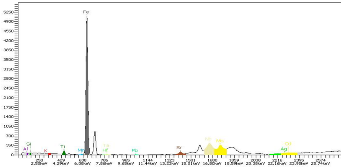
Fig. 1. XRF Spectrum of the Untreated Clay
