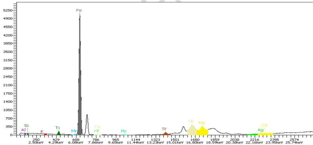
Fig. 2. XRF Spectrum of the treated Clay
