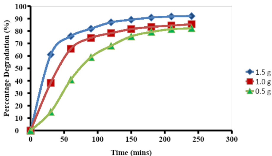
Figure 7: A Graph showing the percentage of degradation of Color Index Blue 194 using MIL-53(AI)
