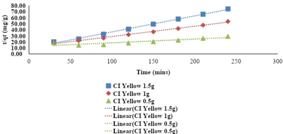
Figure 9: Pseudo-second-order degradation graph of Color Index Yellow 145
