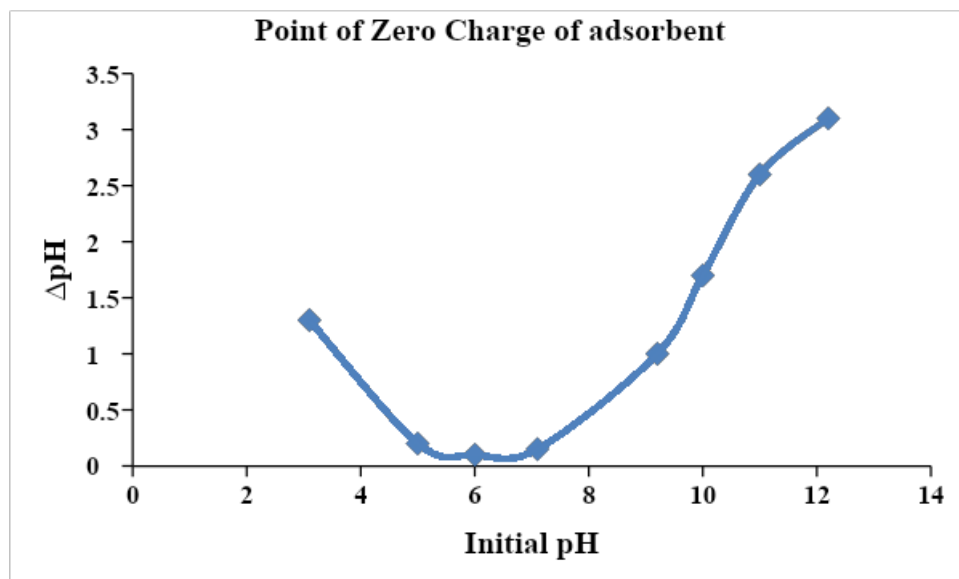
Figure 4: Point of Zero charge of MIL-53(Al)
