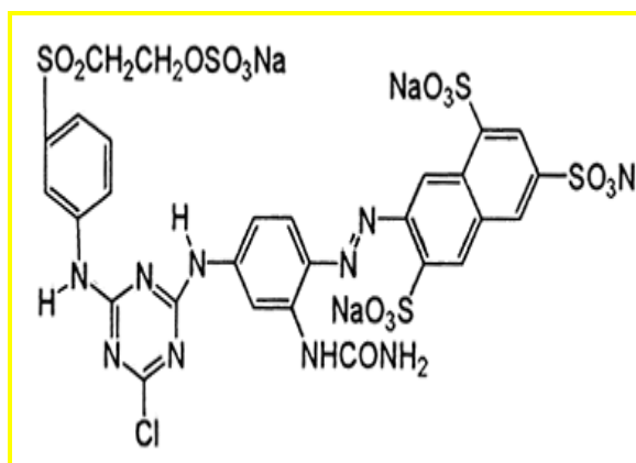
Figure 1: Chemical structure
