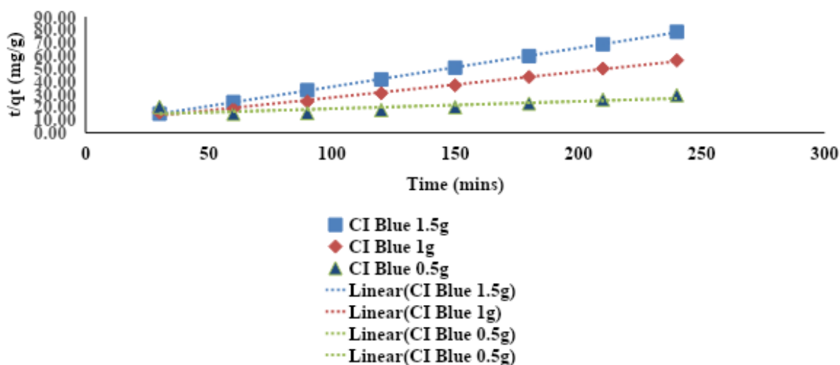
Figure 11: Pseudo second-order degradation graph of color index Blue 194 using MIL-53(Al)
