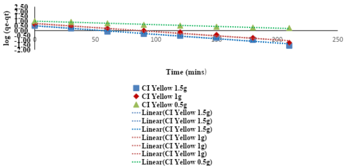
Figure 8: Pseudo-first-order degradation graph of Color Index Yellow 145 using MIL-53(Al)
