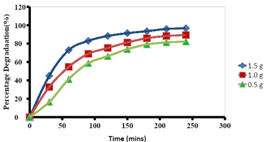
Figure 6: Percentage of degradation of Color Index Yellow 145
