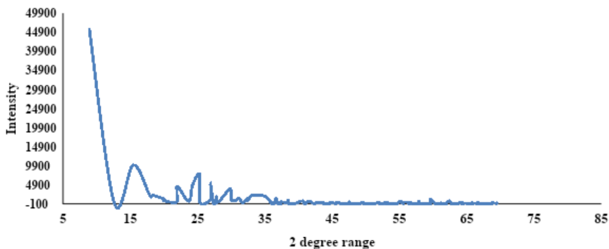
Figure 3: X-ray Diffraction pattern of MIL-53(Al)
