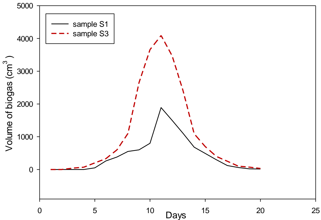
Fig.4.1. A graph of the daily Volume of biogas ( \text{cm}^3 ) collected for sample S_1 and S_3 of the tea substrates for 20 days.
