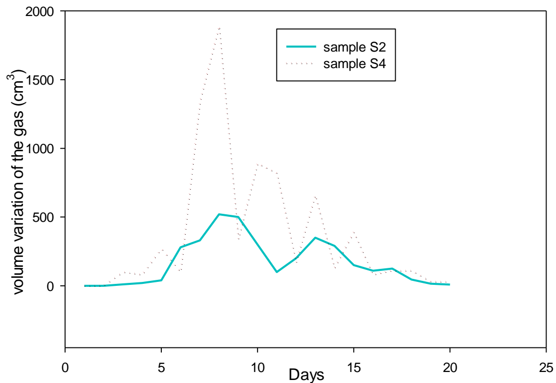
Figure 4.4 shows a graph of daily variation of volume of a gas collected for sample S 2 and sample S 4 for 20 days
