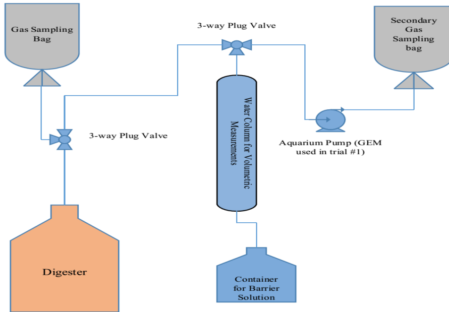
Fig. 3.1 Schematic of bench-scale system for biogas analysis in the laboratory. (Gamble 2014)
