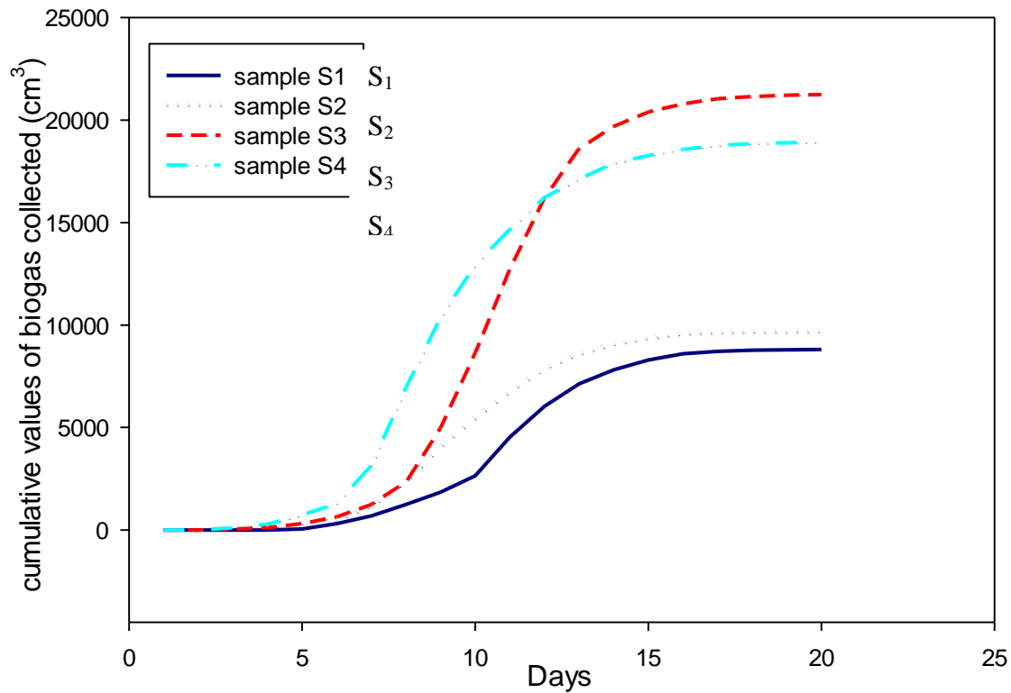
Figure 4.5 shows the cumulative values of biogas collected in 20 days
