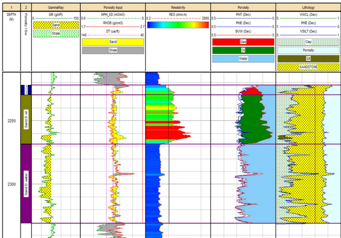
Figure 0.11: Petrophysical Plot of TMG-02 shows the fluid in Sand D as having oil with a gas cap.
