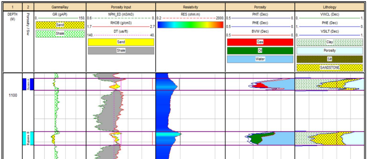
Figure 0.9: Petrophysical plot of TMG-02 shows the fluid in Bypass A and B
