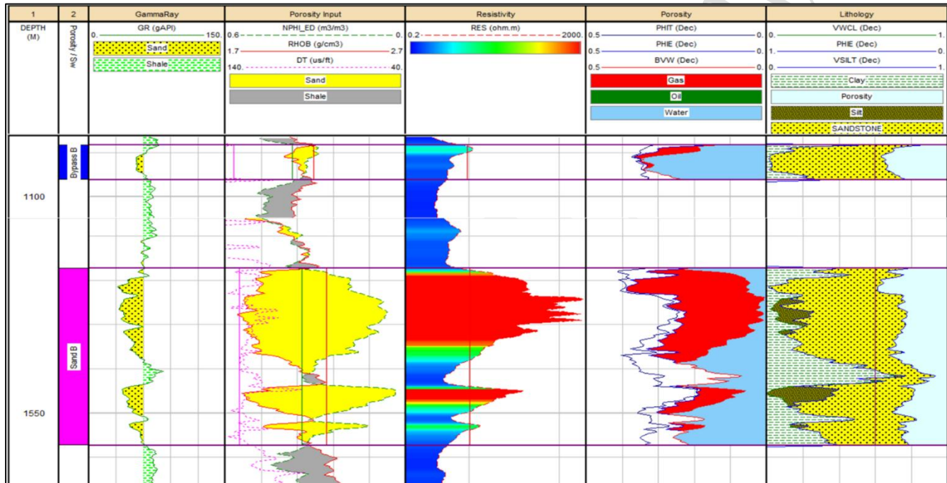
Figure 0.13: Petrophysical plot of TMG-03 shows the hydrocarbon in Bypass B as gas and Sand B as gas.
