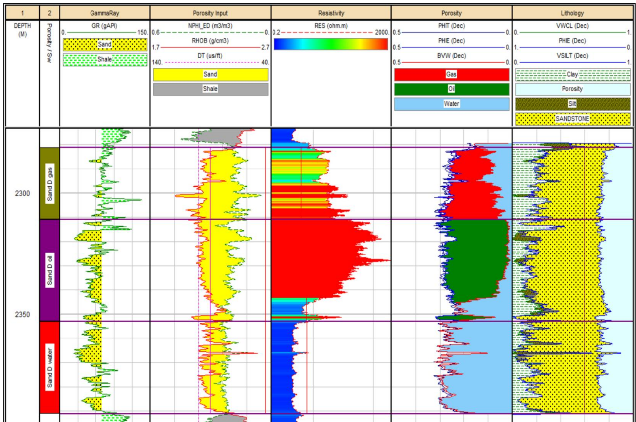
Figure 0.19: Petrophysical plot of TMG-05A shows the hydrocarbon in Sand D as oil with a gas cap.
