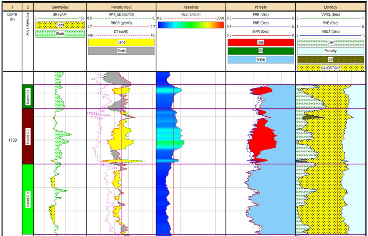
Figure 0.14: Petrophysical plot of TMG-03 shows the hydrocarbon in Sand C as gas.
