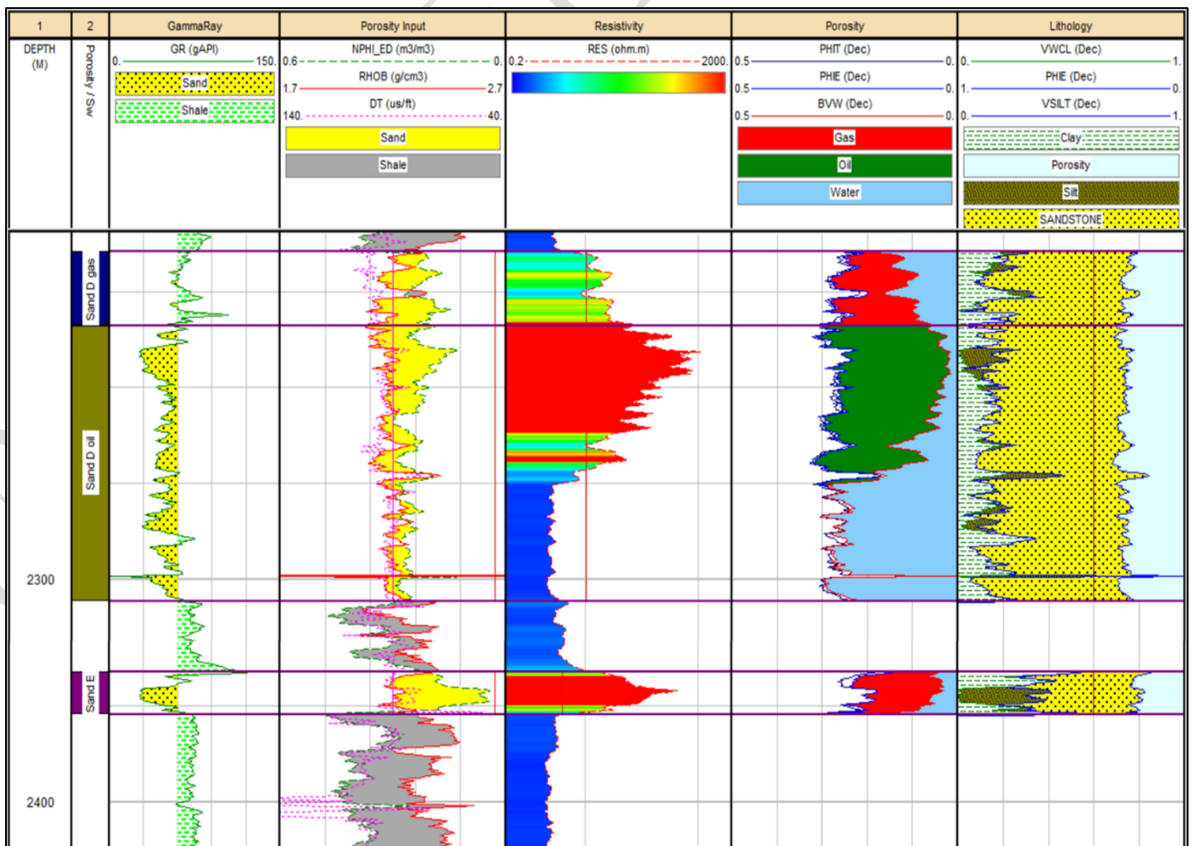
Figure 0.15: Petrophysical Plot of TMG-03 shows the hydrocarbon in Sand D as oil with gas gap and Sand E as gas.
