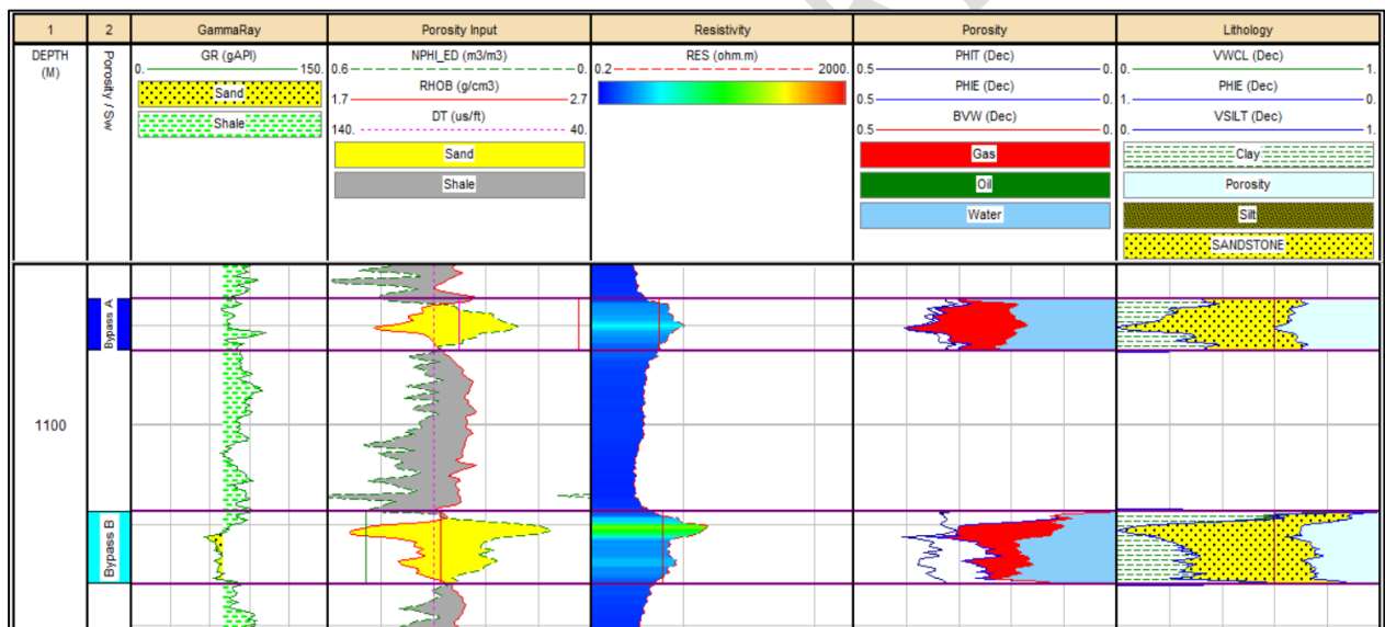
Figure 0.16: Petrophysical Plot of TMG-05A showing the hydrocarbon in Bypass A and B as gas
