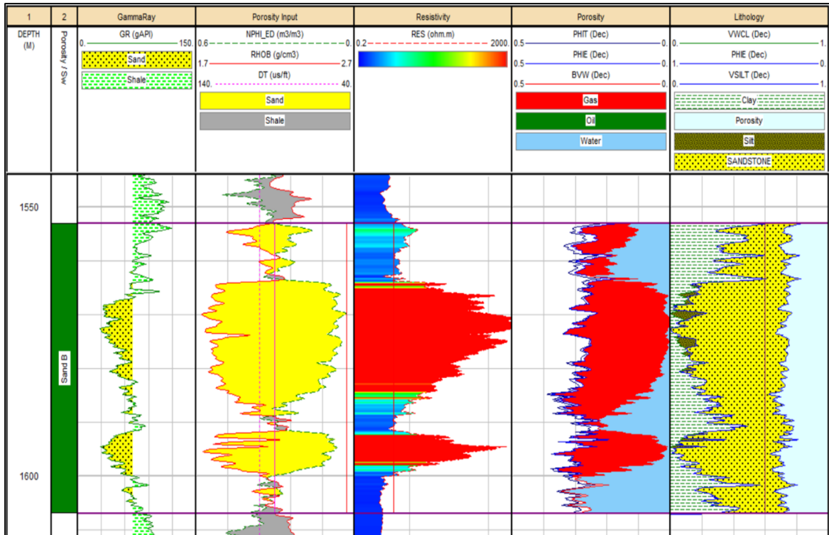
Figure 0.17: Petrophysical plot of TMG-05A showing the fluid in Sand B as Gas.
