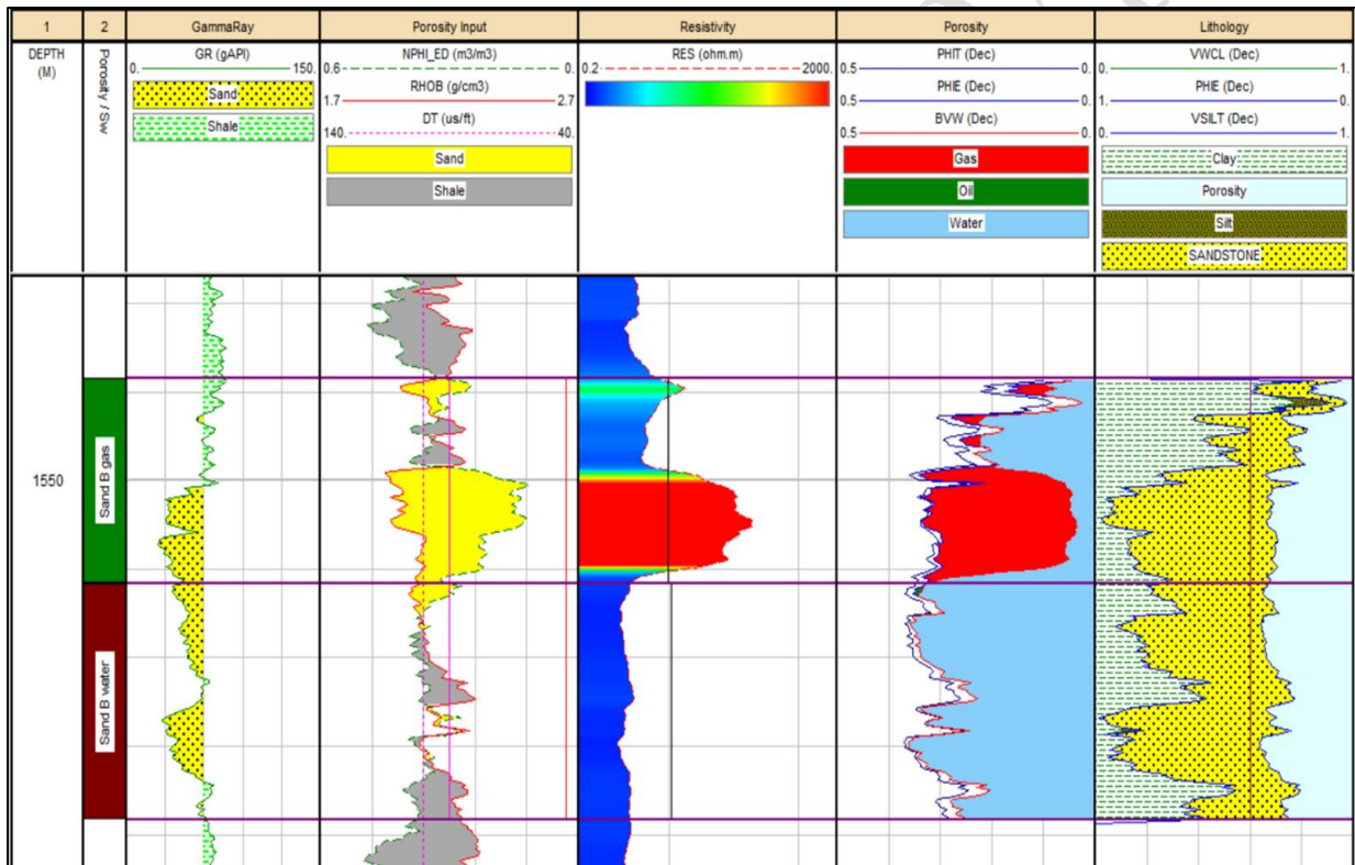
Figure 0.10: Petrophysical Plot of TMG-02 shows the in Sand as Gas
