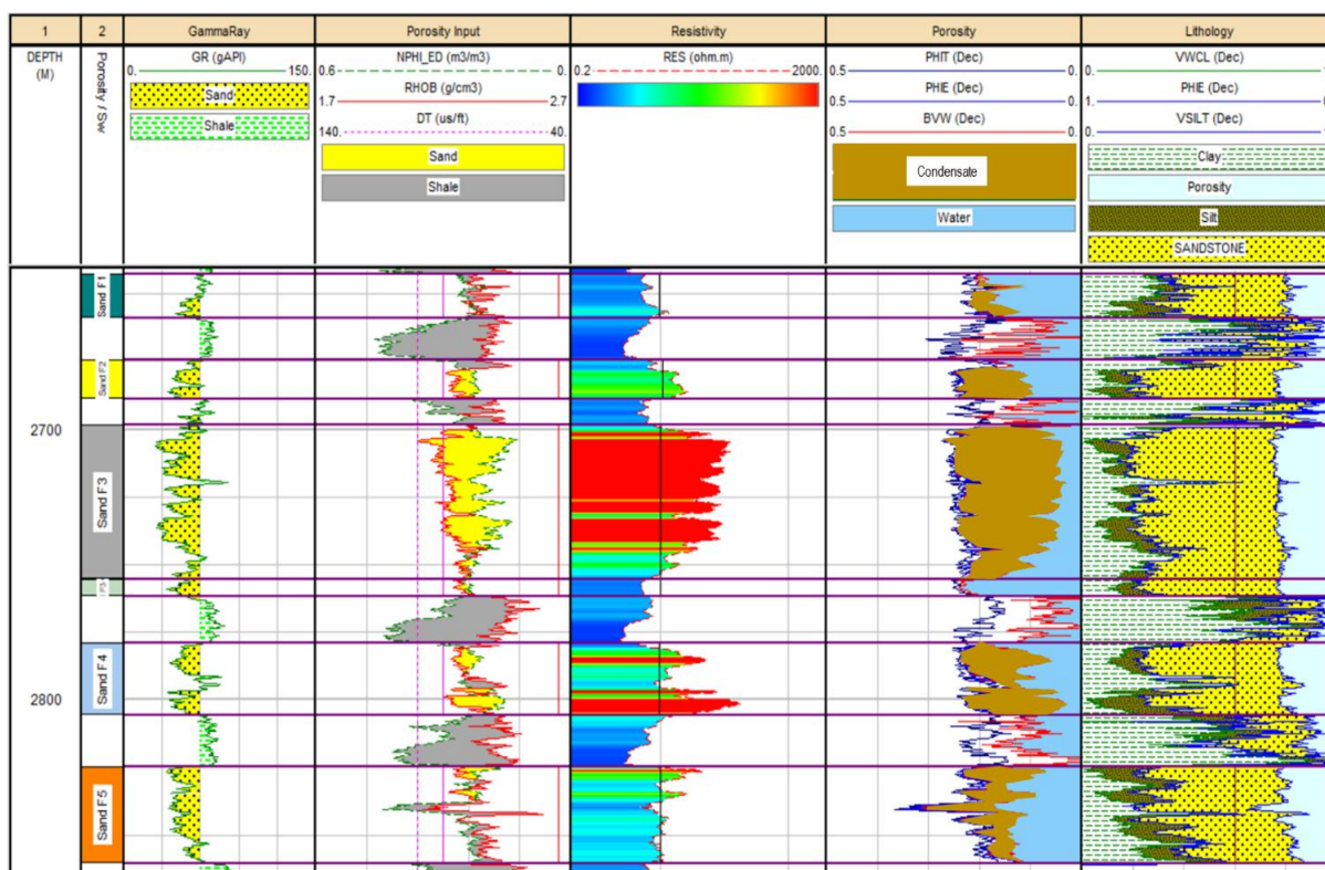
Figure 0.12: Petrophysical plot of TMG-02 showing the Gas condensate saturation within the Sand F subdivided reservoir.
