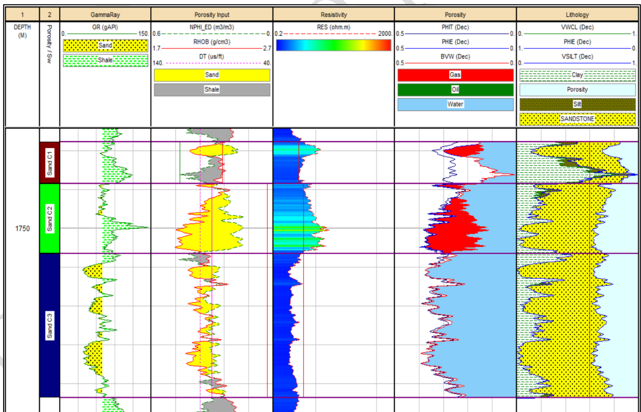
Figure 0.18: Petrophysical plot of TMG-05A shows the hydrocarbon in Sand C as Gas.
