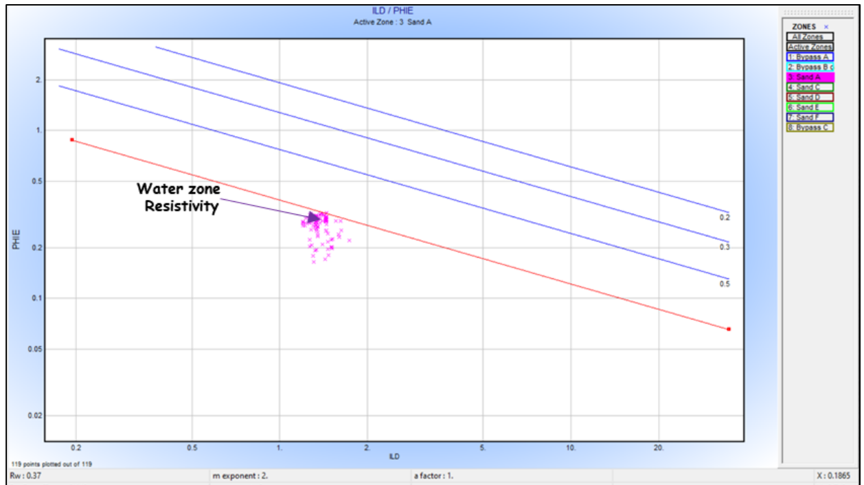
Figure 0.3: R_w estimation using Pickett plot for a zone that is completely saturated with water
