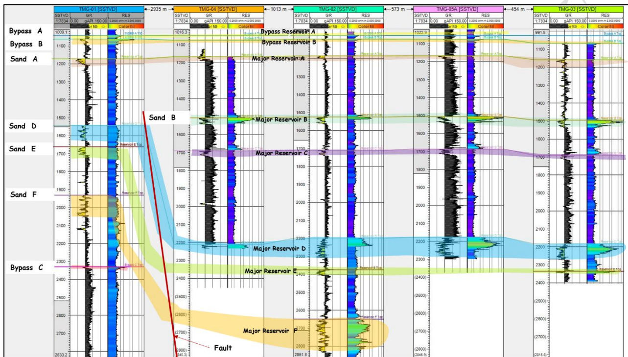
Figure 0.1: Reservoir Correlation of the Major and Identified bypassed Reservoirs.
