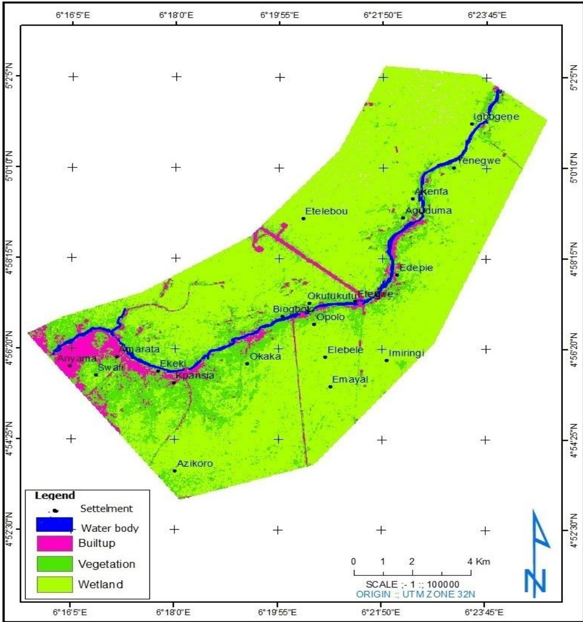
Figure .2: Classified Landsat – OLI imagery of 1990 of the study area.
