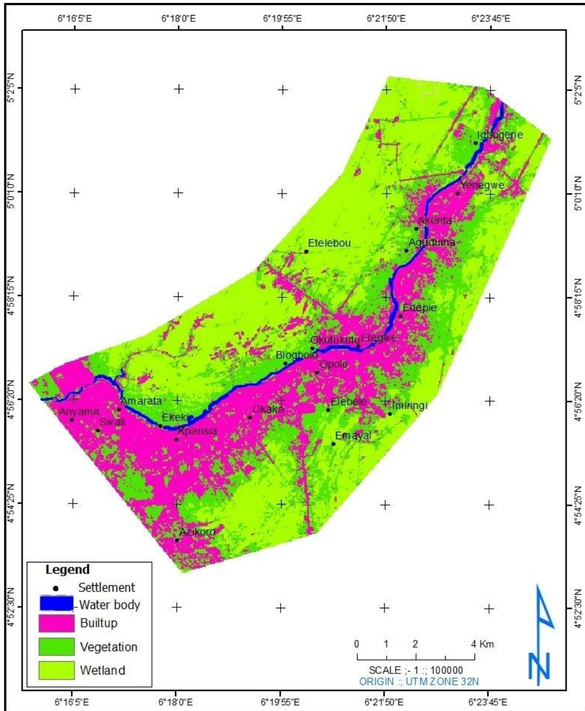
Figure 4: Classified imagery of 2010 of the study area. (Source: Author's Field Work, 2021)
