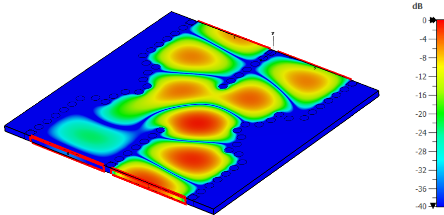
Figure 6: E-Field distribution of the analyzed coupler.
