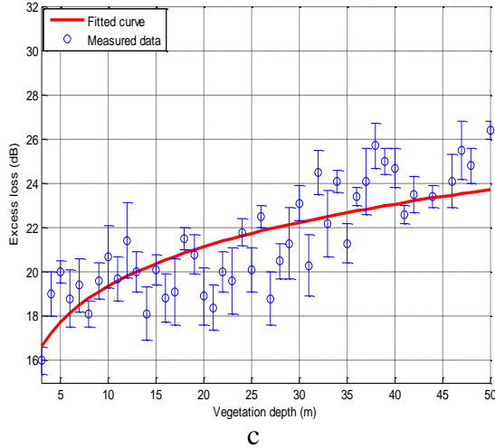
Figures 8a&b Excess loss for ‘inside geometry’ fitted with a curve using the combined data at 3.5 GHz and 5.0 GHz Figures 8c&d Excess loss for ‘into geometry’ fitted with a curve using the combined data at 3.5 GHz and 5.0 GHz
