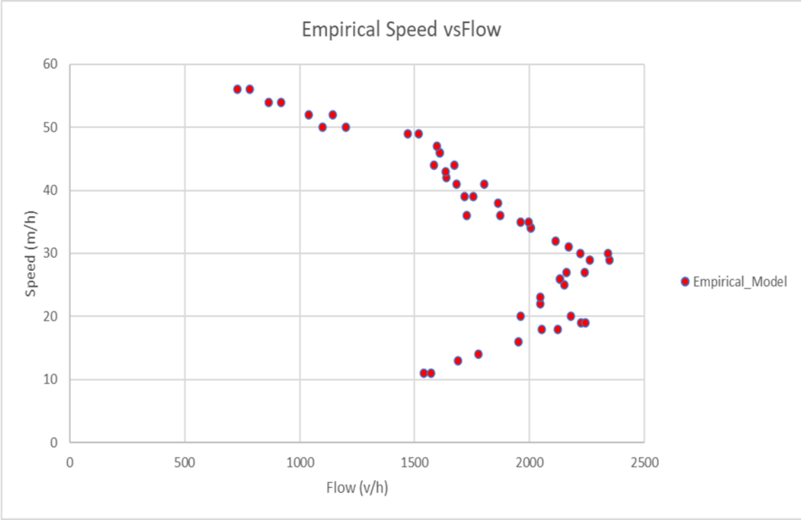
Figure 5: Empirical Speed vs Flow Curve
