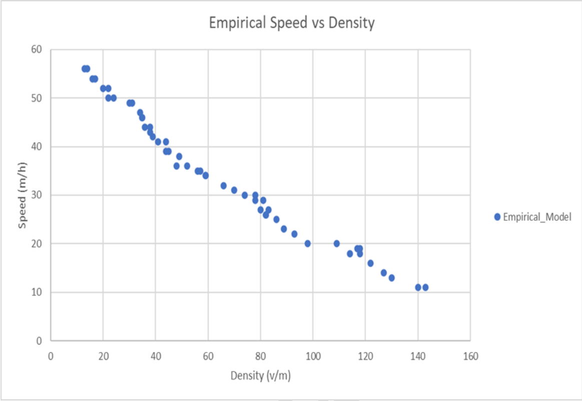
Figure 4: Empirical Speed vs Density Curve
