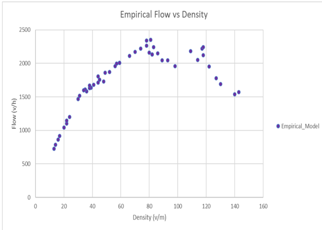
Figure 6: Empirical Flow vs Density Curve
