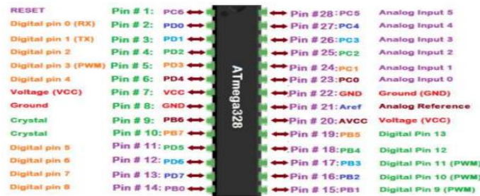
Fig. 3. Pinout diagram of ATmega-328
