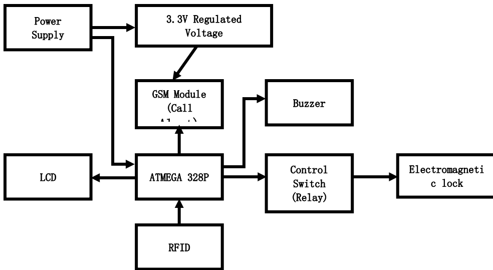
Fig. 2: Block Diagram
