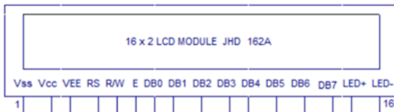
Fig 4: Schematic of 16x2 Liquid Crystal Display (LCD) Module
