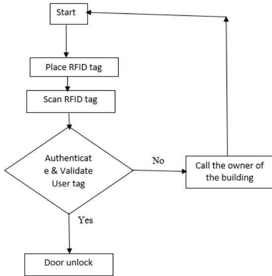
Fig. 1: System Flowchart
