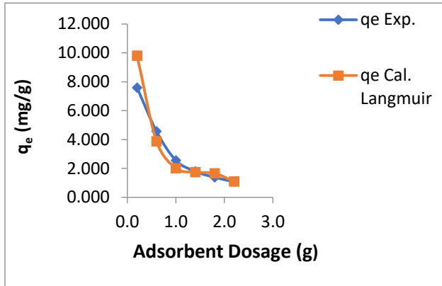
Figure 1: Langmuir plot of q_{e-Exp} Vs q_{e-Cal}
