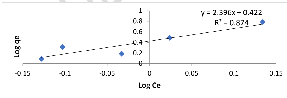
Figure 3: Freundlich Adsorption Isotherm for Removal of lead (II) with CPTAC.
