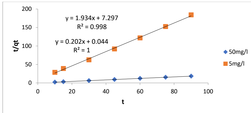
Figure 4: Pseudo-second order kinetic Plot for Removal of lead (II) with CPTAC at varying conditions
