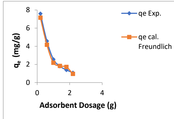
Figure 2: Freundlich plot of q_{e-Exp} Vs q_{e-Cal}
