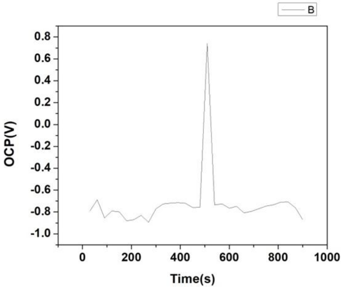
Fig. 4. Open Circuit Potential (OCP) against Time
