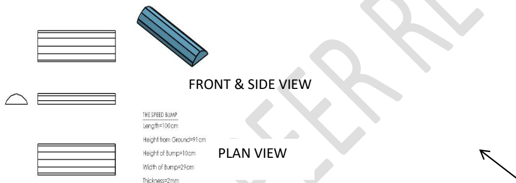
Figure.4 Front, Side and Plan View of the Speed Bump
