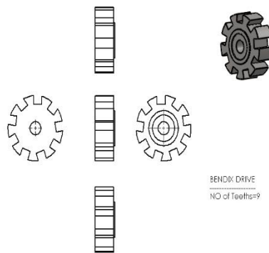
Figure.7 The Front, Side and Plan view of Bendix Teeth
