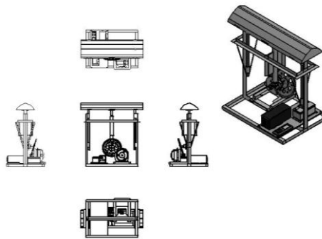
Figure .2 Front, Plan and Side View of Speed Breaker Generator
