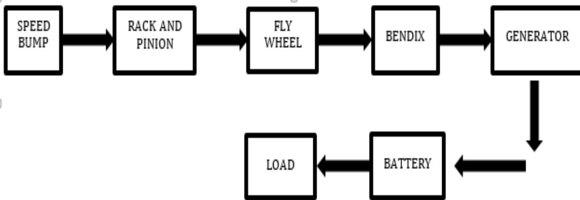
Figure.3 block schematics of the Speed Breaker Generator Model
