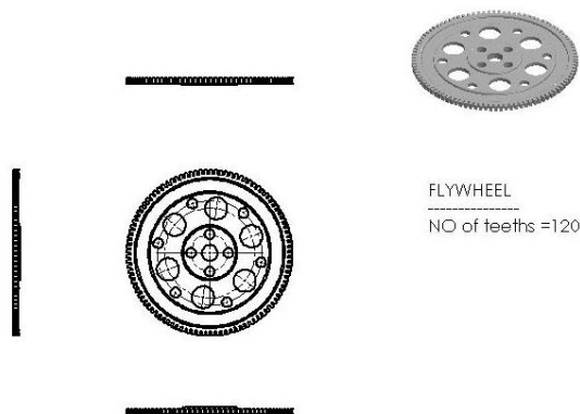
Figure.5 Front, Side and Plan view of Flywheel
