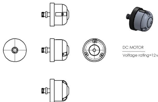
Figure.9 The Front, Side and Plan View of the Generator
