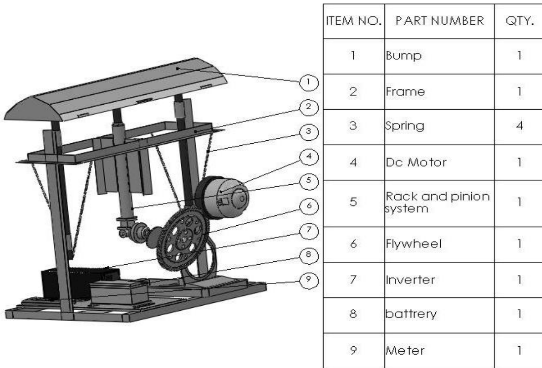
Figure.1 the Speed Breaker Generator
