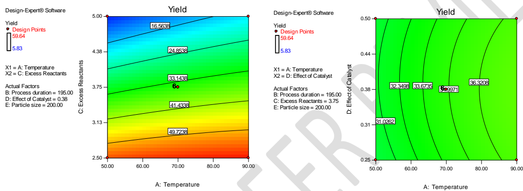
Figure 9: The contour plots for excess reactants against temperature and yield of BAC and the contour plots for the effect of catalyst against temperature and yield of BAC
