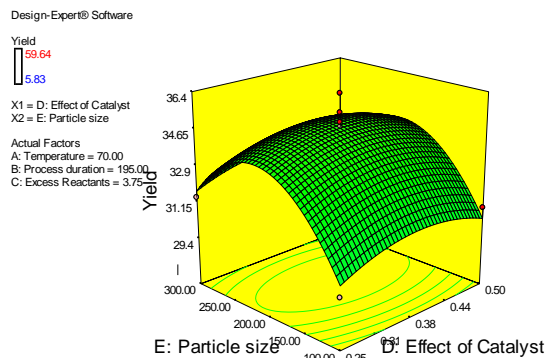
Figure 24: The 3 - D Plot for particle size against yield and excess reactants of BAC and the 3 - D Plot for particle size against yield and effect of catalyst of BAC
