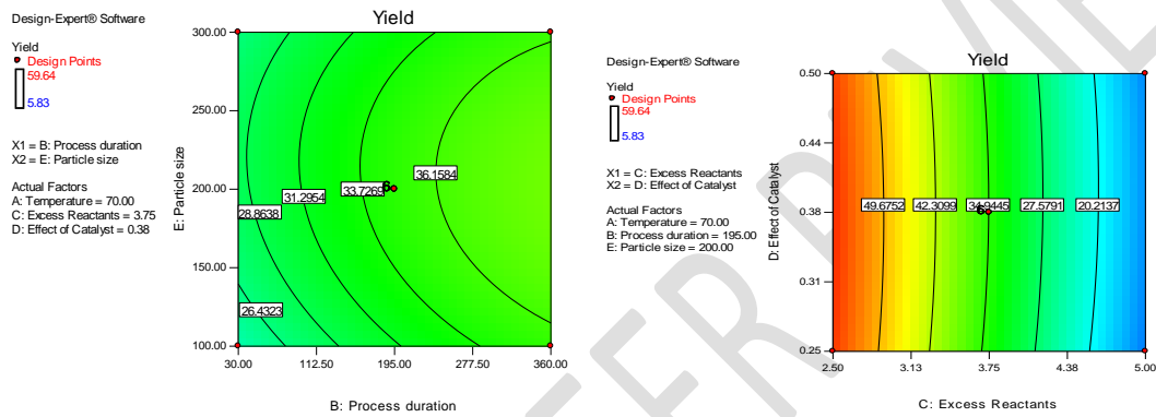
Figure 6: The contour plots for particle size against process duration and yield of BAC And the contour plots for the effect of catalyst against excess reactant and yield of BAC
