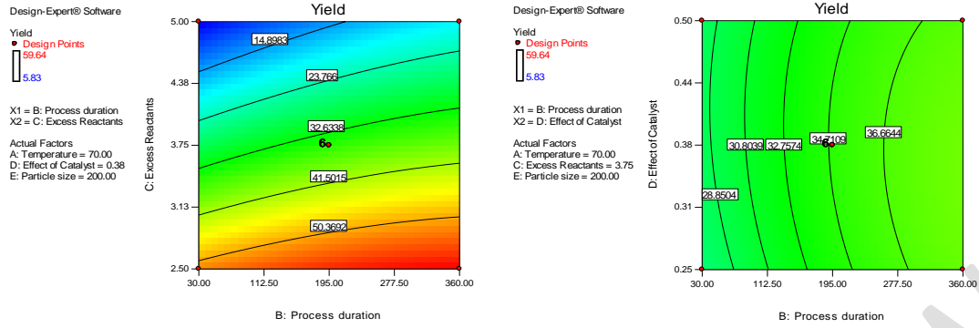
Figure 5: The contour plots for excess reactants against process duration and yield of BAC and contour plots for the effect of catalyst against process duration and yield of BAC
