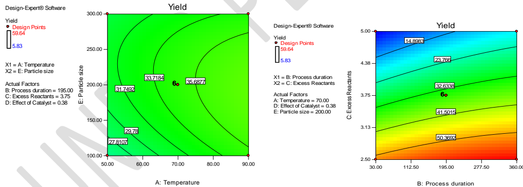
Figure 10: The contour plots for particle size against temperature and yield of BAC and the contour plots for excess reactant against process duration and yield of BAC
