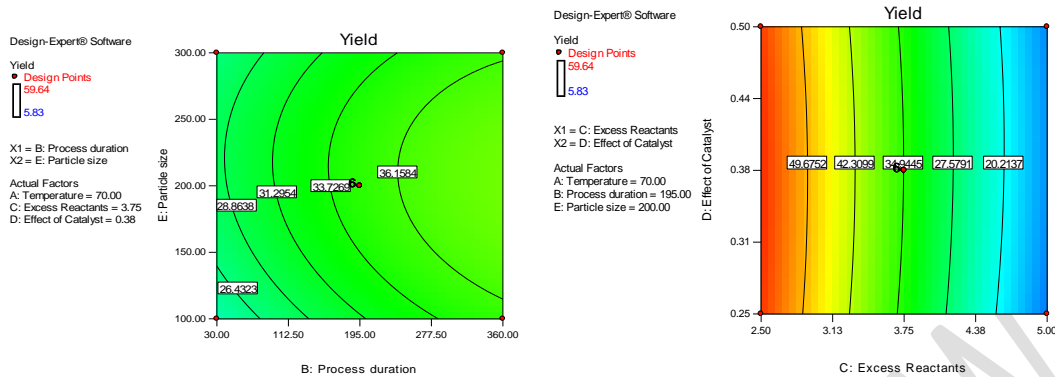
Figure 17: The contour plots for particle size against process duration and yield of BAC and the contour plots for the effect of catalyst against excess reactants and yield of BAC
