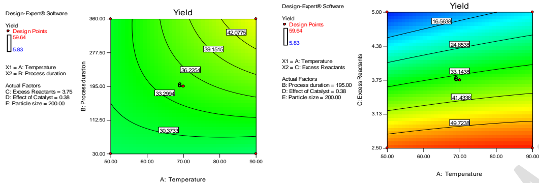
Figure 14: The contour plots for process duration against temperature and yield of BAC and the contour plots for excess reactants against temperature and yield of BAC
