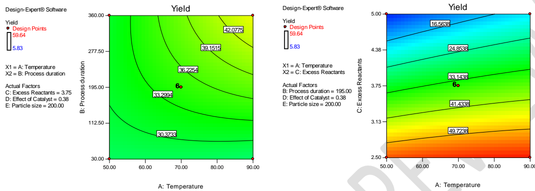
Figure 3: The contour plots for process duration against temperature and yield of BAC and The contour plots for excess reactants against temperature and yield of BAC
