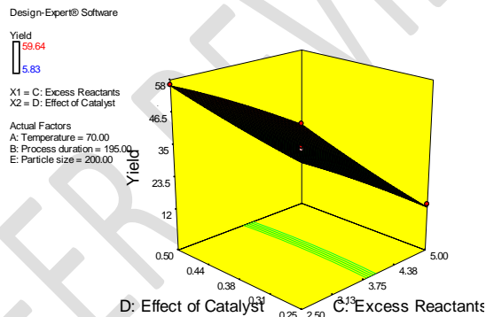
Figure 23: The 3 - D Plot for particle size against process duration and yield of BAC and The 3 - D Plot for the effect of catalyst against yield and excess reactants of BAC and
