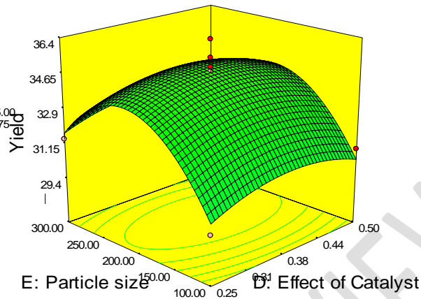
Figure 19: The 3 - D Plot for particle size against yield and effect of catalyst of BAC
