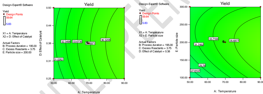
Figure 4: The contour plots for the effect of catalyst against temperature and yield of BAC and The contour plots for particle size against temperature and yield of BAC
