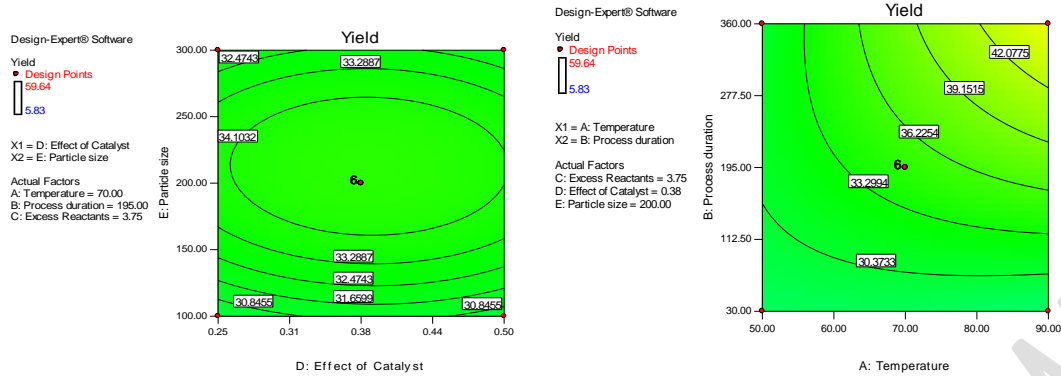
Figure 8: The contour plots for particle size against the effect of catalyst and yield of BAC and the contour plots for process duration against temperature and yield of BAC
