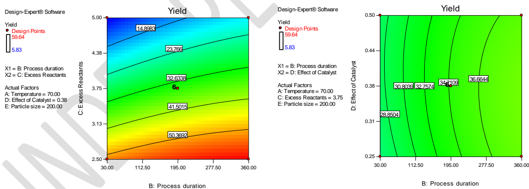
Figure 16: The contour plots for excess reactants against process duration and yield of BAC and the contour plots for effect catalyst against process duration and yield of BAC
