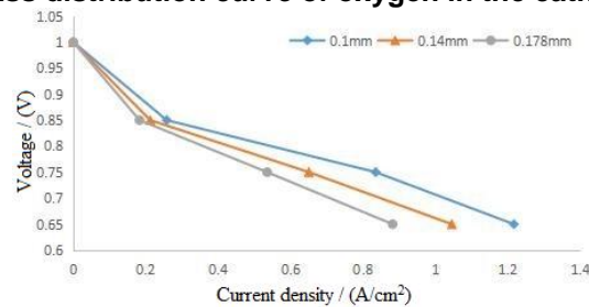
Fig. 17. Polarization curves of different proton exchange membranes
