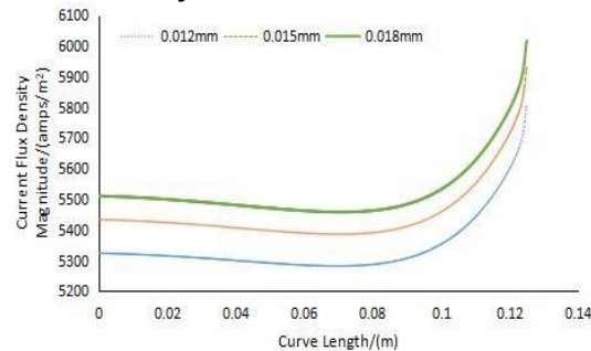
Fig. 13. Current density distribution at the intermediate section
