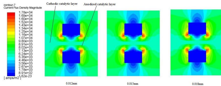
Fig. 13. Current density distribution at the intermediate section
