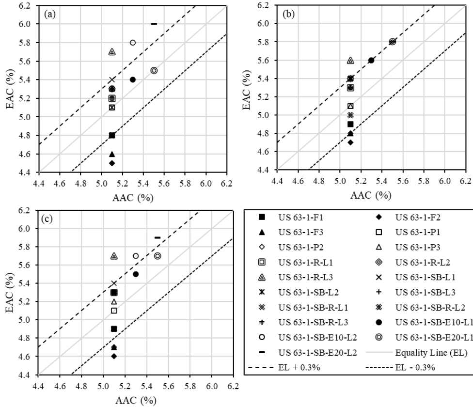
Fig. 9. AAC% versus EAC% values for the US 63-1 mixes; (a) AMMDM, (b) CMMDM, and (c) AACMMDMs
