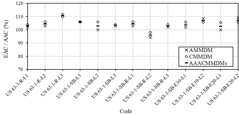
Fig. 13. EAC per AAC values for the US 63-1 lab mixes
