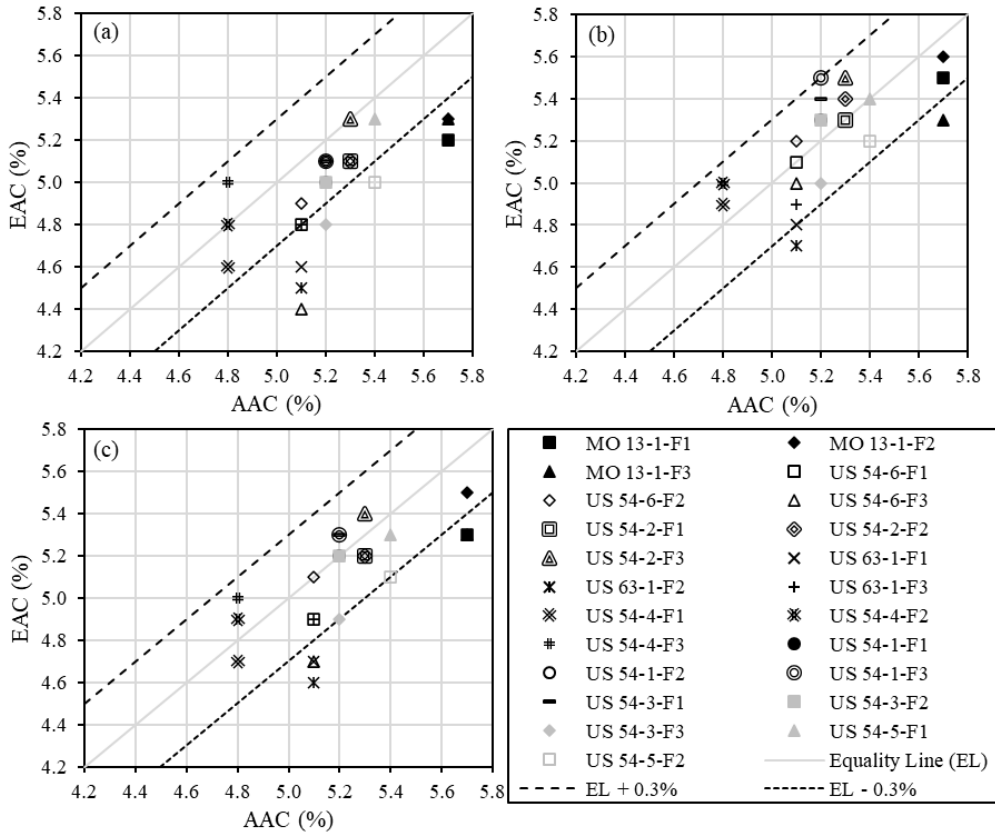
Fig. 15. AAC% versus AAC% values for field mixes constructed in 2016; (a) AMMDM, (b) CMMDM, and (c) AAACMMDMs
