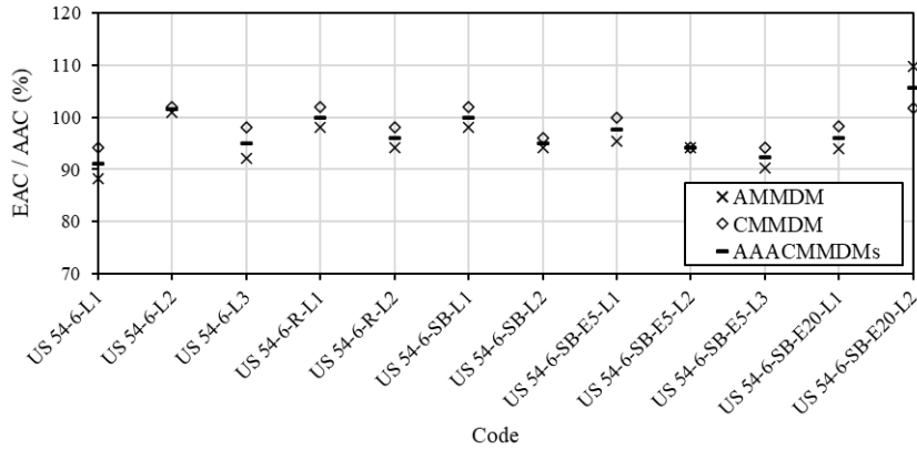
Fig. 11. EAC per AAC values for the US 54-6 lab mixes
