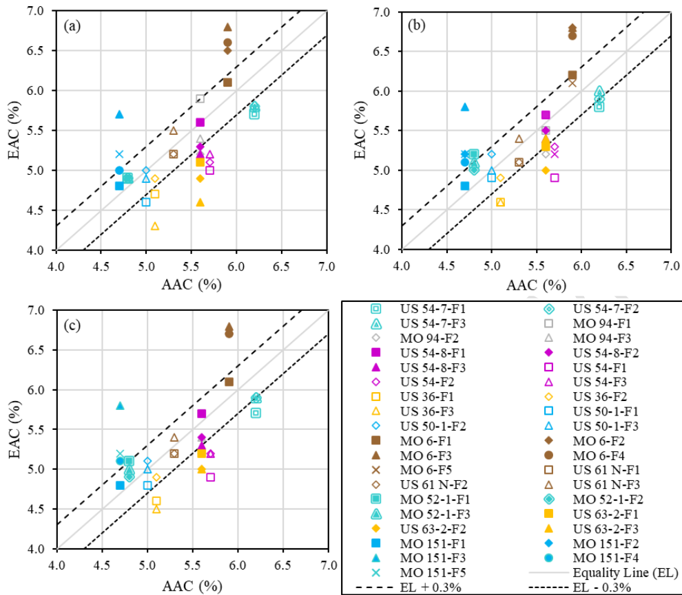
Fig. 6. AAC% versus EAC% values for field mixes constructed before 2016; (a) AMMDM, (b) CMMDM, and (c) AACMMDMs
