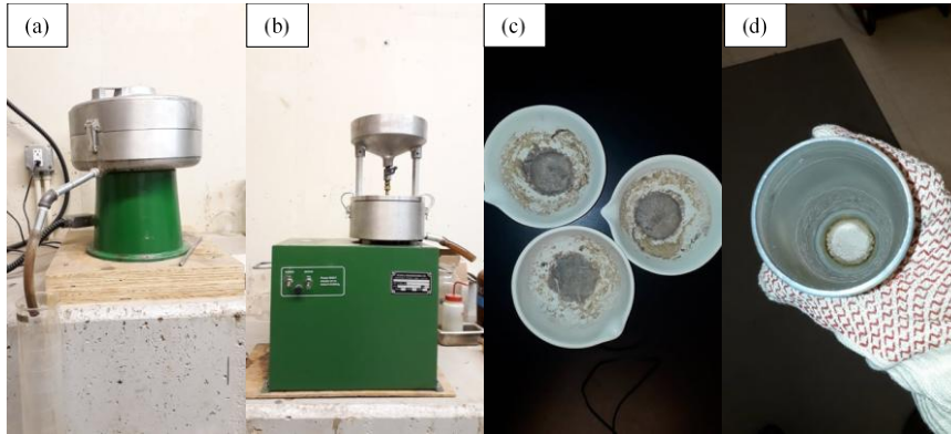
Fig. 3. (a) Centrifuge extractor, (b) Filterless centrifuge, (c) Mineral matter in ignition dishes, and (d) Mineral matter in centrifuge metal cup [5]
