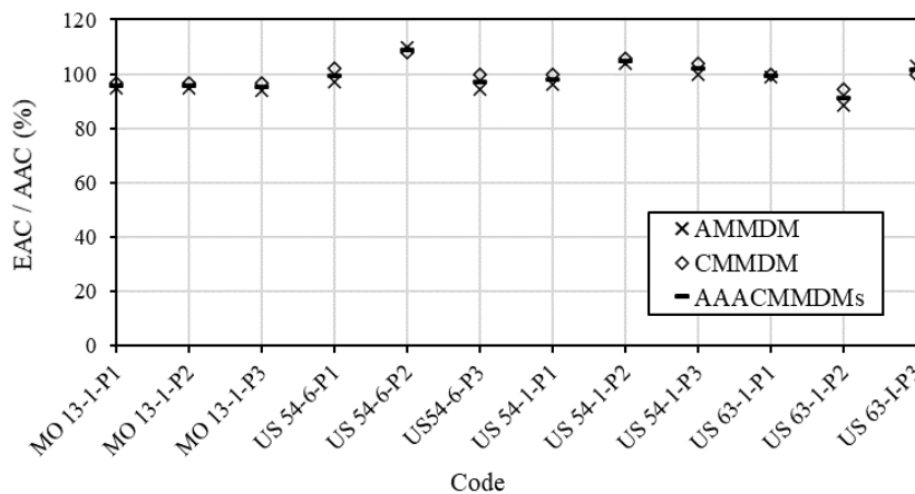
Fig. 5. EAC per AAC values for plant mixes
