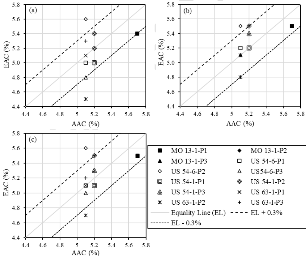
Fig. 4. AAC% versus EAC% values for plant mixes; (a) AMMDM, (b) CMMDM, and (c) AACMMDMs
