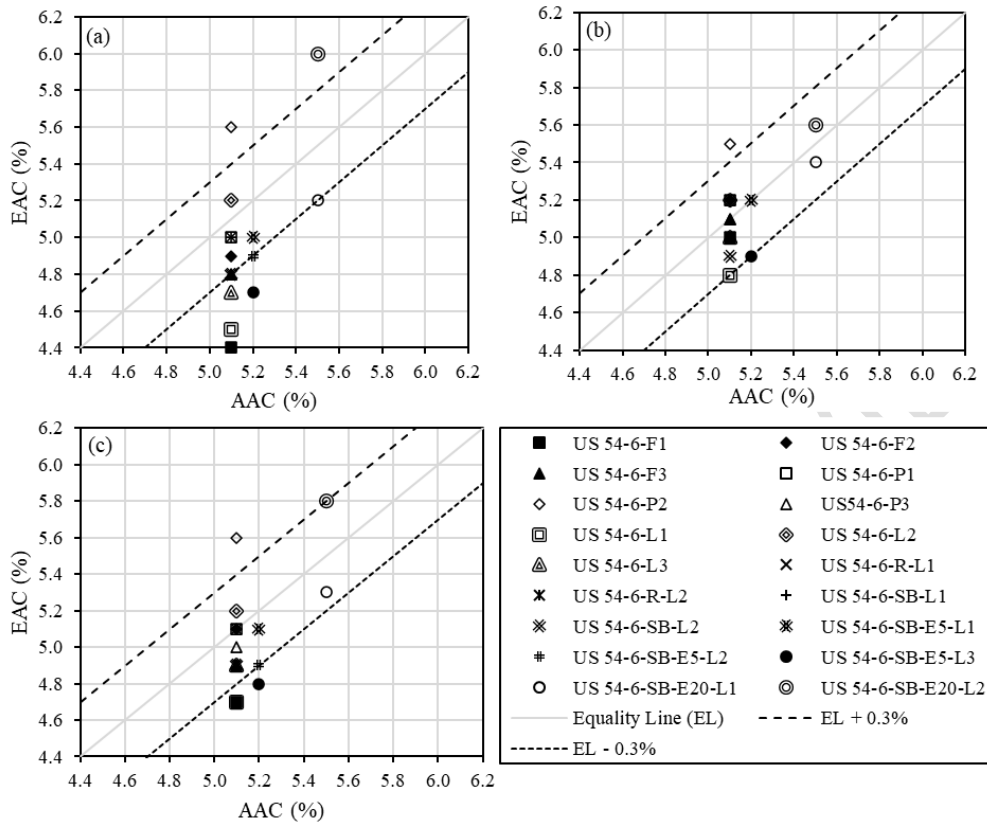
Fig. 8. AAC% versus EAC% values for the US 54-6 mixes; (a) AMMDM; (b) CMMDM, and (c) AACMMDMs
