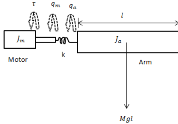
Figure 2: Flexible joint model of the manipulator
