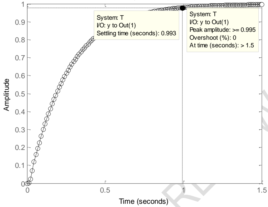
Figure 6: Step response of the mixed synthesis controlled flexible joint model
