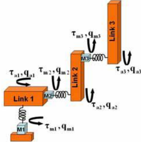
Figure 1: A flexible joint dynamic model with 6 DOF [17]
