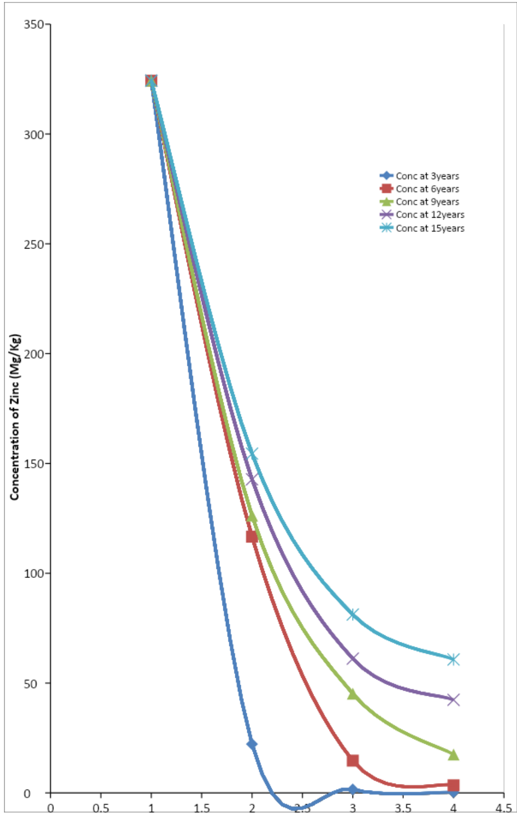
Figure 3: Graphical plot of Zinc concentration at Varying Time Steps.
