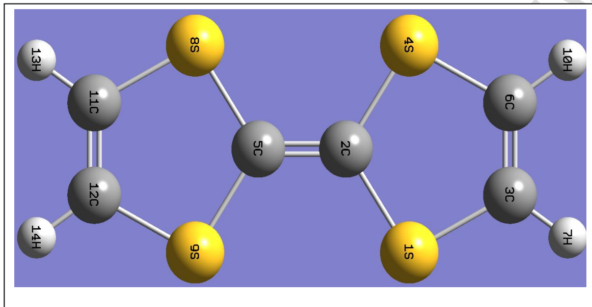
Figure 1: optimized structure of TTF
