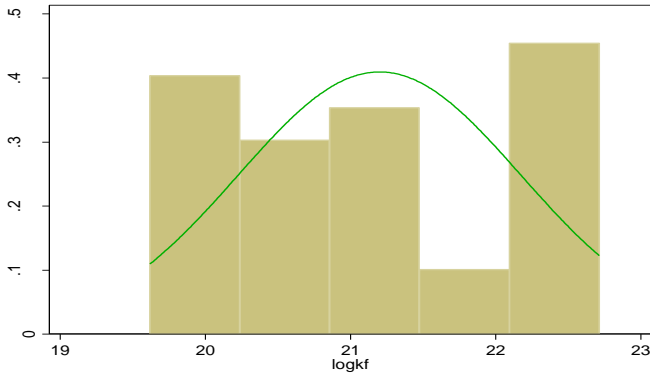
Figure 1: Histogram with a Density Plot of “Logkf”
