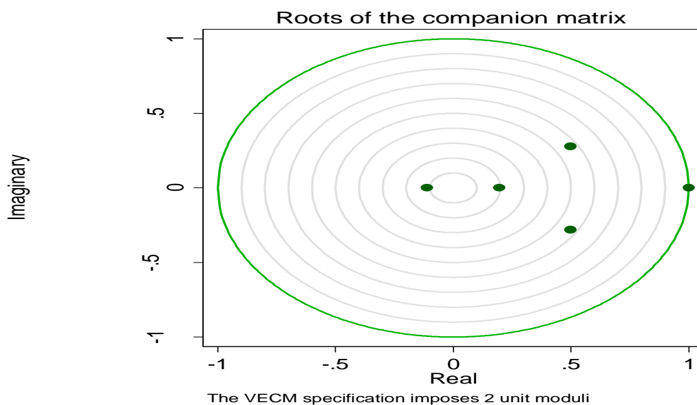
Figure 5: Roots of the Companion Matrix after VECM
