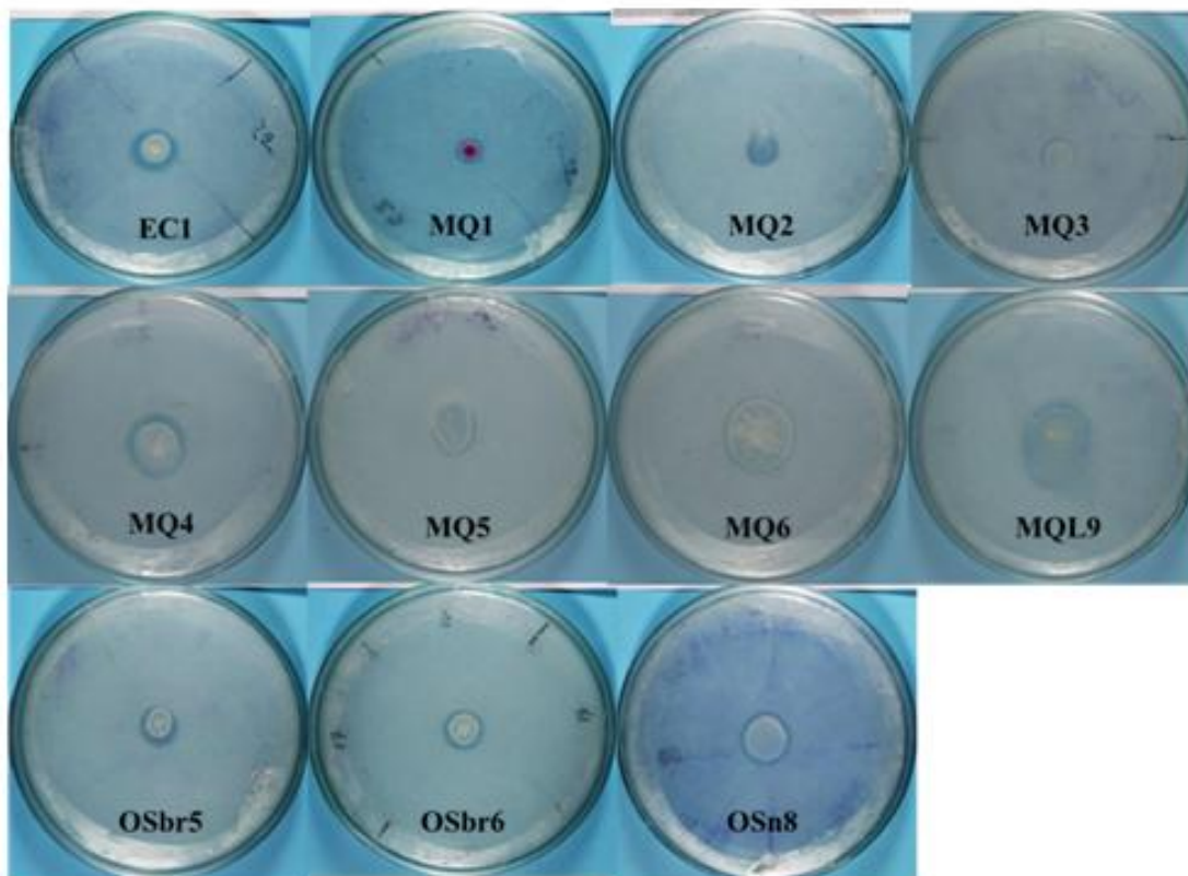
Plate 1: Solubilization of inorganic ZnO in vitro by eleven rhizobacterial isolates after 5 days of incubation at 28±1°C. The formation of halo zone around the bacterial colonies demonstrated the solubilization of zinc oxide.
