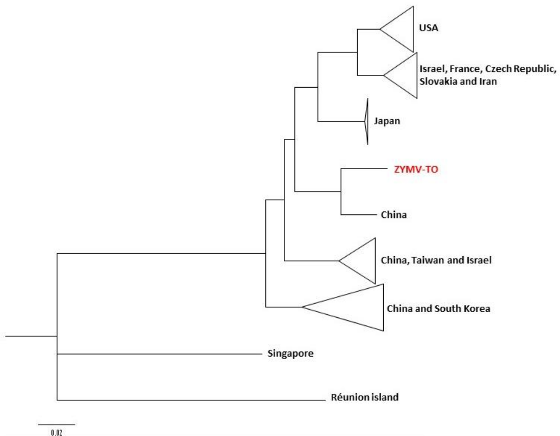
Figure 2: Phylogenetic analysis of ZYMV-TO. Phylogenetic tree showing ZYMV-TO and 63 complete nucleotide sequences of the ZYMV viral genome. Built by the Maximum Likelihood method, PhyML 3.0 program. The bar at the bottom of the left side shows the number of substitutions/sites. The tree was rooted by midpoint . Some branches were collapsed for better visualization.
