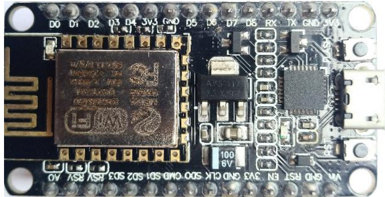
Fig. 5 NodeMCU ESP8266 board
