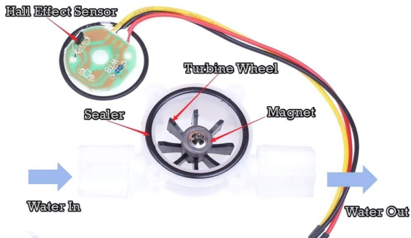
Fig. 4 Internal components of water flow sensor
