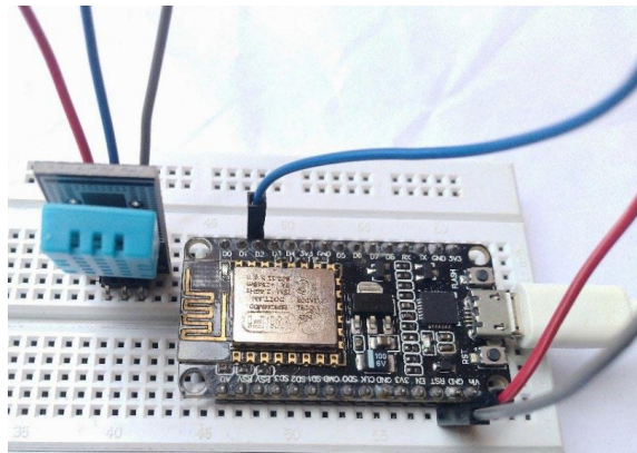
Fig. 12 Interfacing DHT11 sensor to NodeMCU
