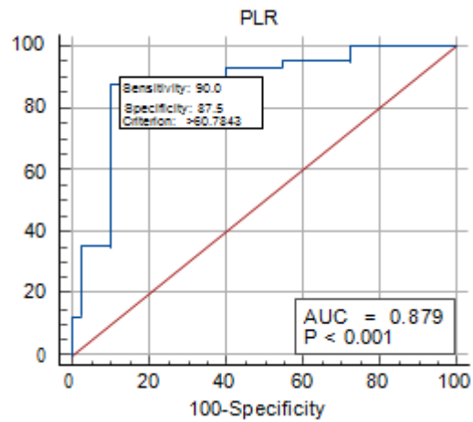
Figure (8): ROC curve of PLR
