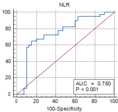
Figure (7): ROC curve of NLR
