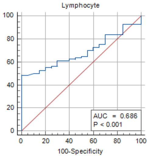
Figure (1): ROC curve of lymphocyte PLR
