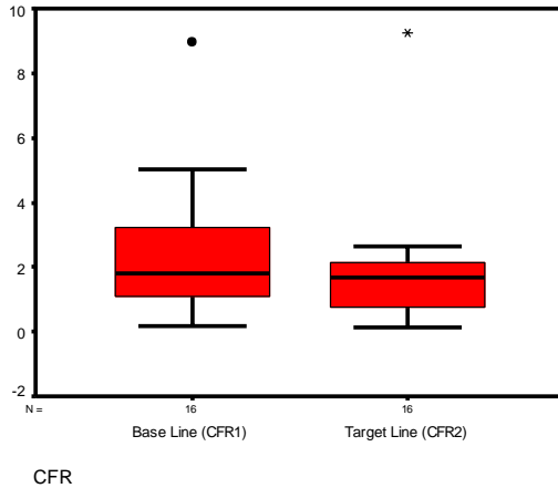
Fig 1: Box-Whisker plot
