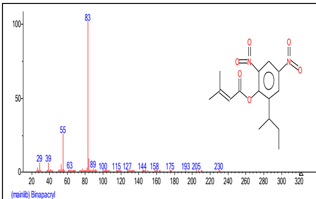
Fig. 2i. Mass spectrum of Binapacryl structure.
