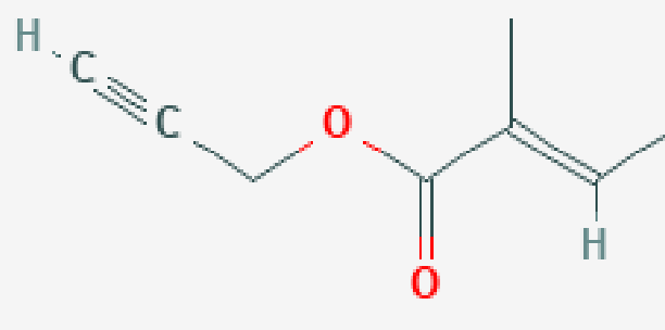
Fig. 2n. Structure of Prop-2-ynyl (E)-2-methylbut-2-enoate.
