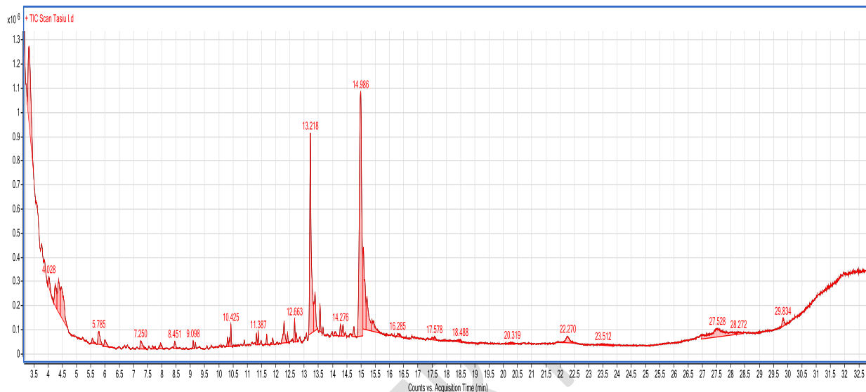
Figure 1: Chromatogram of GC-MS of Gossypium hirsutum cotton seed oil
