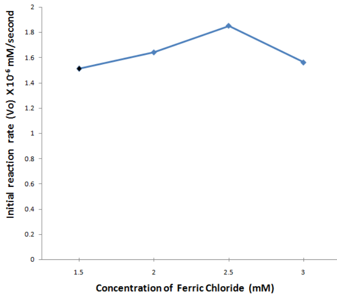
Figure 3: Effect of varying concentrations of ferric chloride on the on the initial reaction rate of TMB oxidation by crude peroxidase from watermelon seeds
