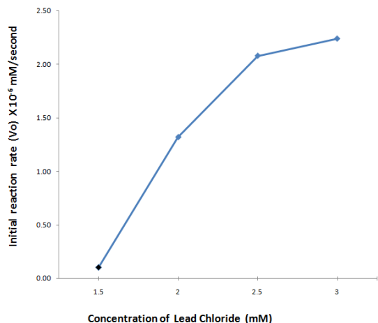
Figure 1: Effect of varying concentrations of lead Chloride on the on the initial reaction rate of TMB oxidation by crude peroxidase from watermelon seeds
