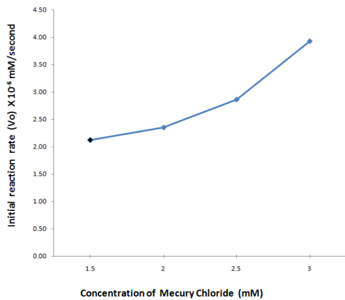
Figure 2: Effect of varying concentrations of Mercury Chloride on the on the initial reaction rate of TMB oxidation by crude peroxidase from watermelon seeds
