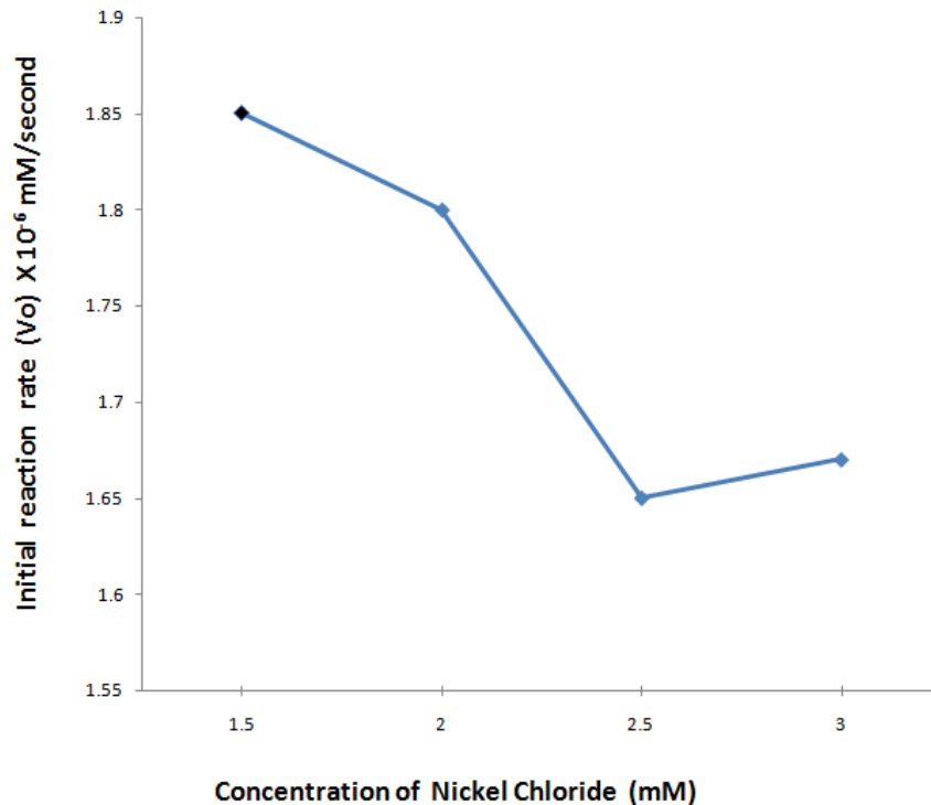
Figure 4: Effect of varying concentrations of nickel Chloride on the on the initial reaction rate of TMB oxidation by crude peroxidase from watermelon seeds
