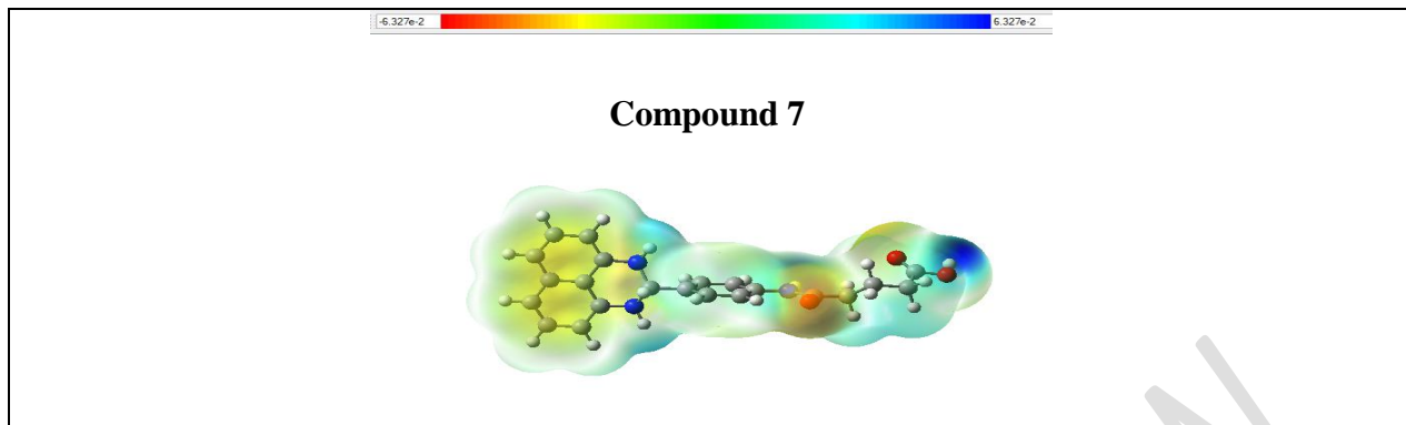
Figure 1: Surface of molecular Electrostatic potentials of 2,3-dihydro-1H-perimidine
