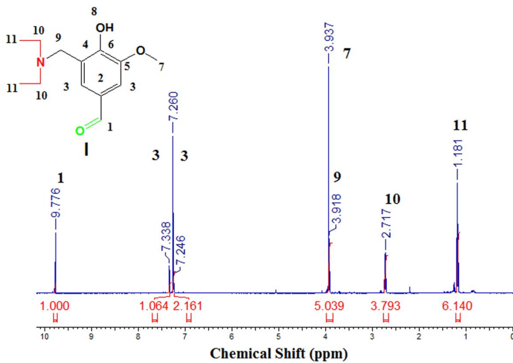
Figure 1: ^1\text{H} NMR ( \text{CDCl}_3 ) of 2-[(diethylamino)methyl]-4-formyl-6-methoxyphenyl acrylate.
