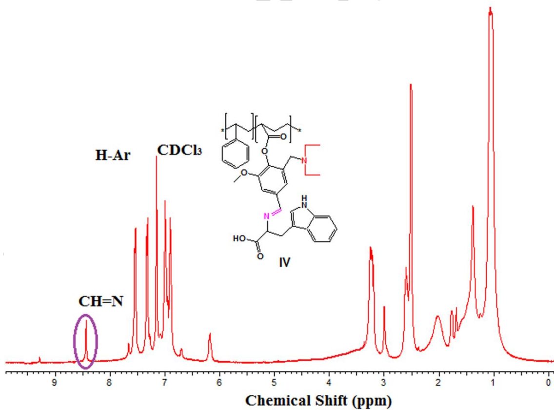
Figure 4: ^1\text{H} NMR spectra (DMSO) of P(styrene-co-DEAMVA)-g-Tryptophan
