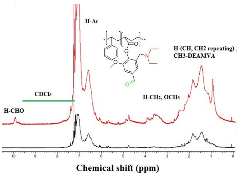
Figure 3: ^1\text{H} NMR spectra ( \text{CDCl}_3 ) of P(S-co-DEAMVA) 10, 25 mole ratio of DEAMVA
