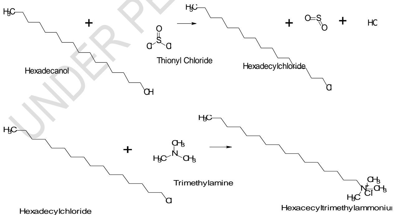
Figure 1. Reaction equations for the synthesis
