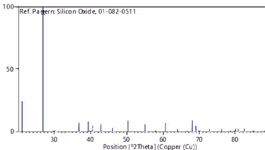
Figure 4e: Stick Pattern showing silicon oxide
