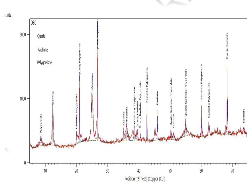
Figure 4b: XRD spectrum of HDTMAC-clay
