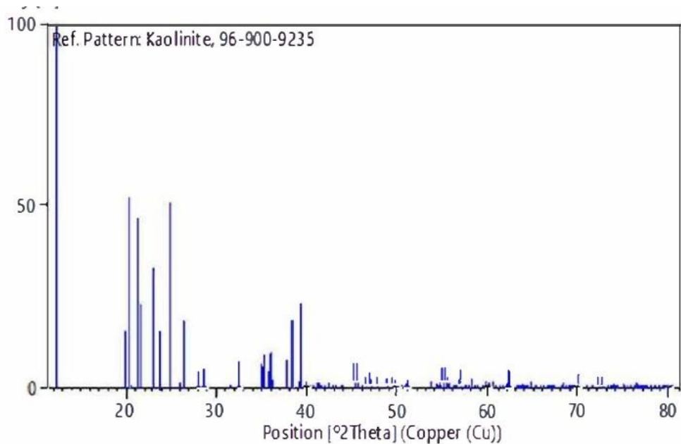
Figure 4c: XRD stick pattern for unmodified kaolinite clay
