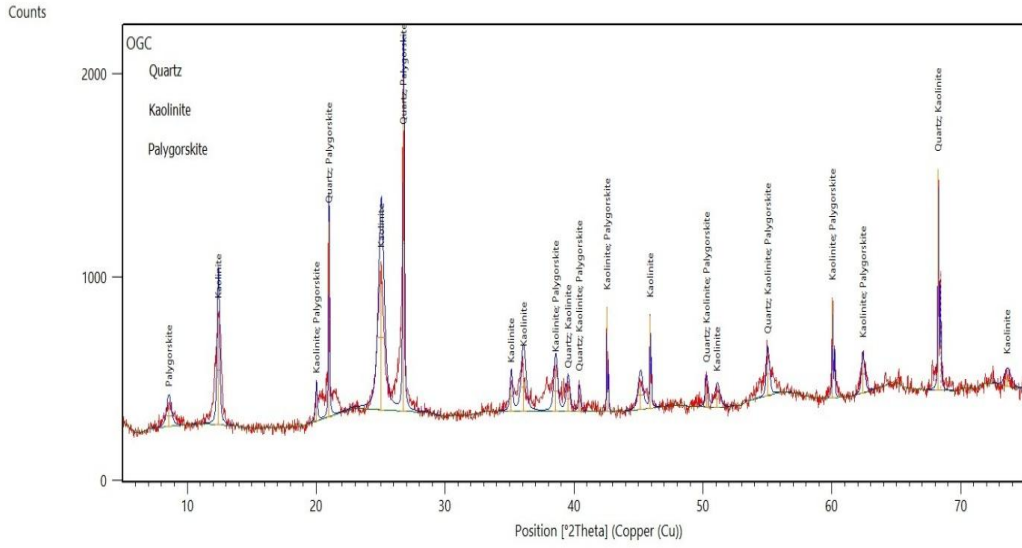
Figure 4a: XRD spectrum of UM-clay
