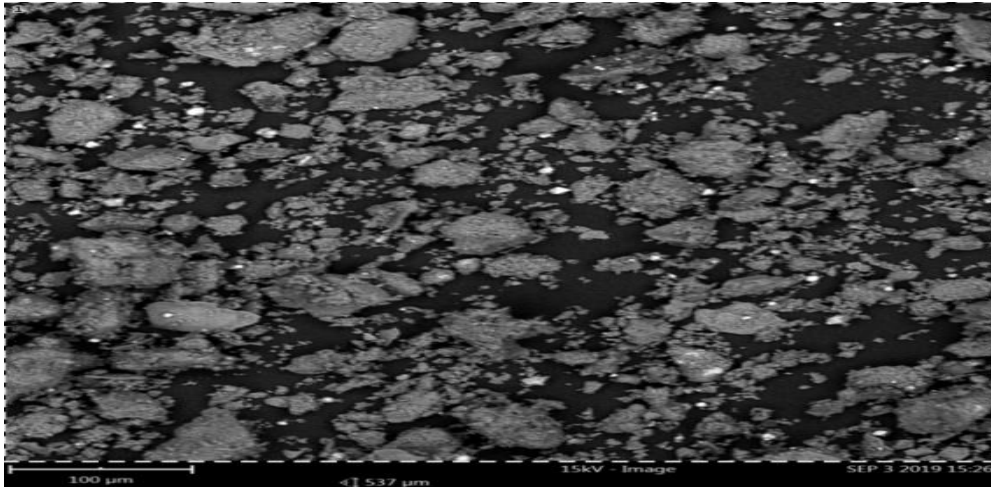
Figure 2a: SEM Image of Unmodified Clay
