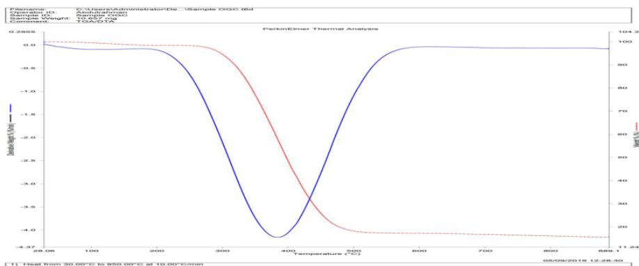
Figure 3a: TGA/DTA of UM-clay
