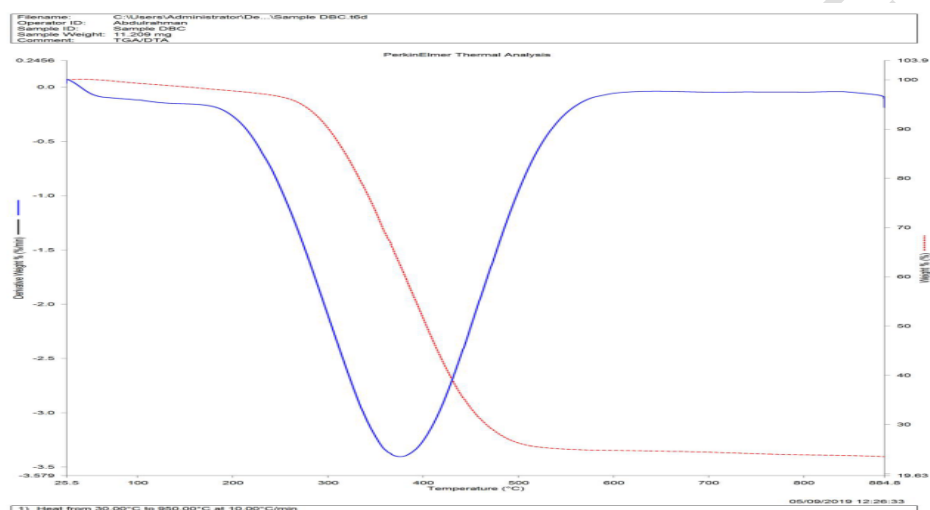
Figure 3b: TGA/DTA of HDTMAC-clay
