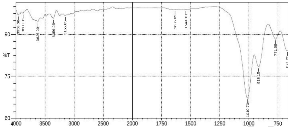
Figure 5a: FTIR spectrum of UM-clay
