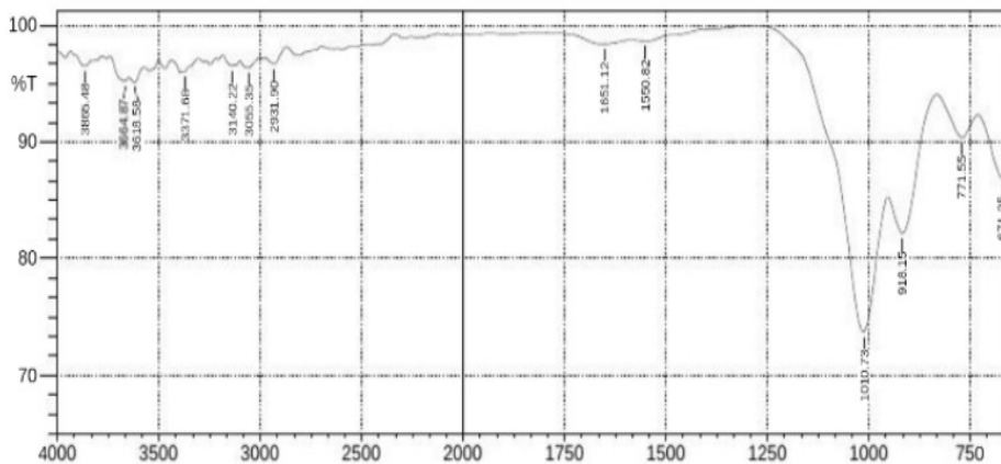
Figure 5b: FTIR spectrum of HDTMAC-clay
