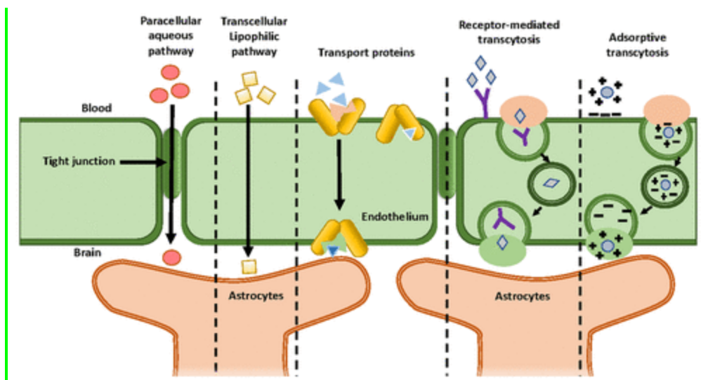
Figure 3. Conventional diagram of the different mechanisms for crossing the blood brain barrier [37].
