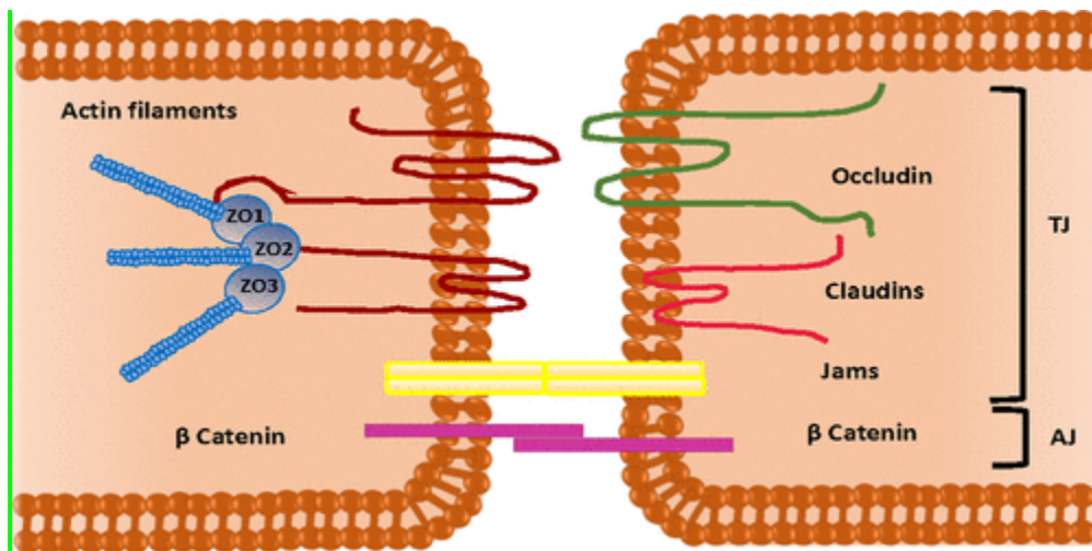
Figure 2. Schematic representation of tight junctions and adherence junctions between endothelial cells [37].
