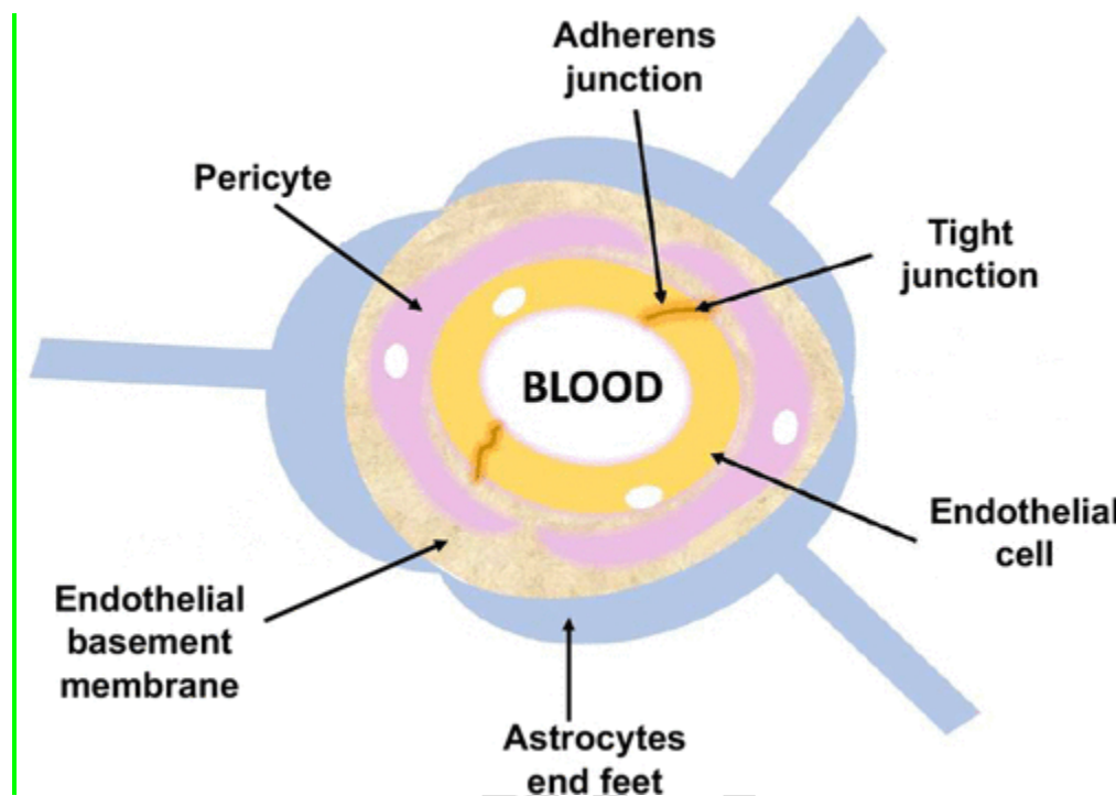
Figure 1. Schematic drawing of the blood brain barrier [37].
