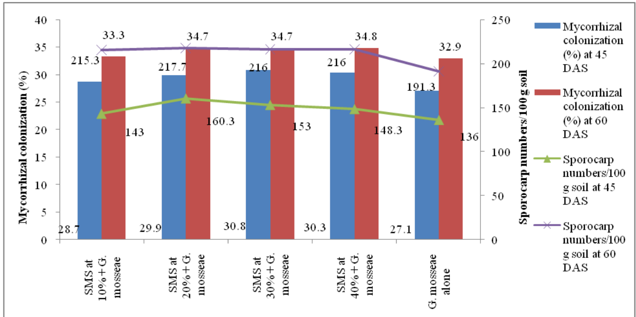
Fig. 1. Effect of spent mushroom substrate on Glomus mosseae establishment in wheat cv. WH 1105
