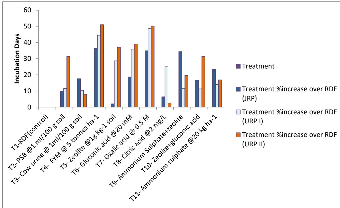
Fig 1.P release pattern at different Incubation days with treatments
