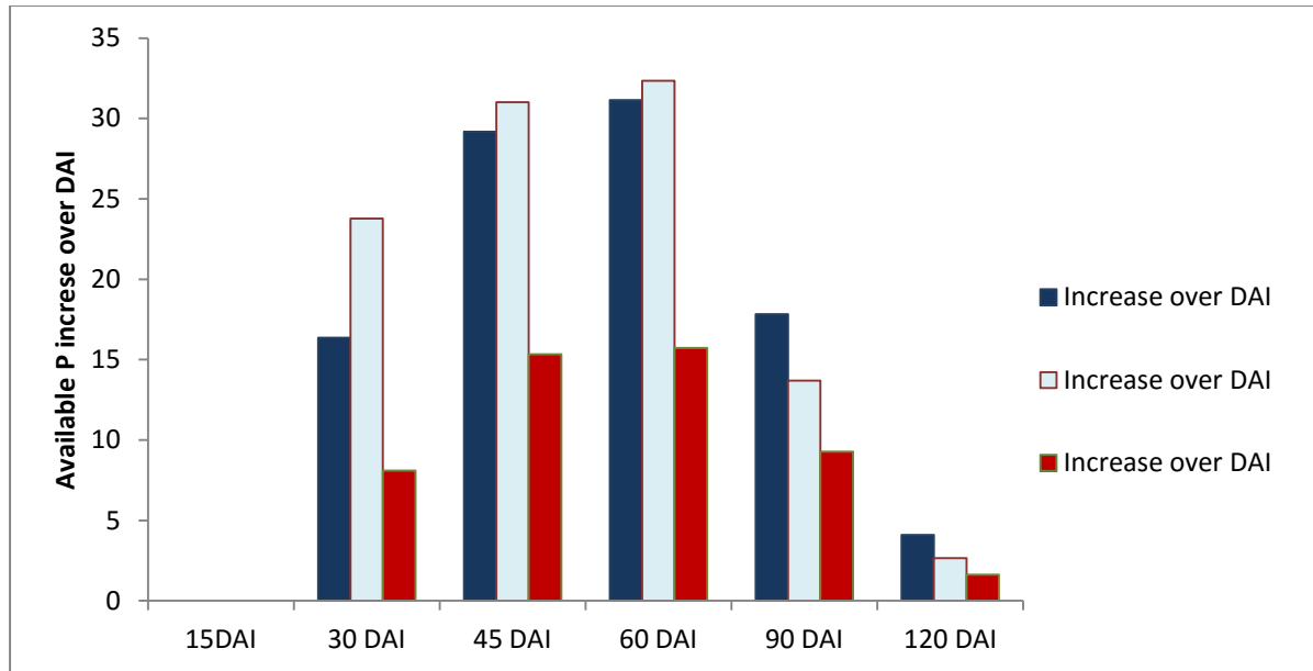
Fig 2. Available Olsen P increase over different DAI
