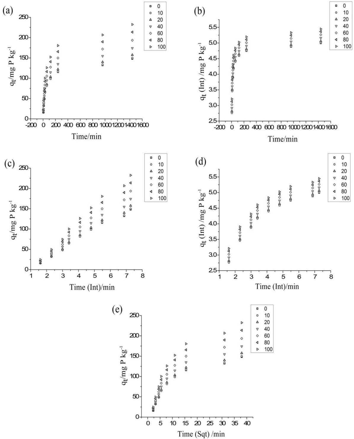
Fig.1. The kinetics of P release by citric acid applied at 0, 10, 20, 40, 60, 80, 100 mM concentrations in highly calcareous soil having 17.5% free CaCO 3 as a function of time and similar data described by five kinetic models: Zero-order ( q_t vs t ) (a), First
