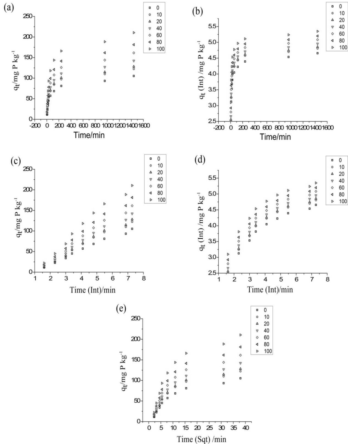
Fig. 2. The kinetics of P release by citric acid applied at 0, 10, 20, 40, 60, 80, 100 mM concentrations in highly calcareous soil having 21.5% free \text{CaCO}_3 as a function of
