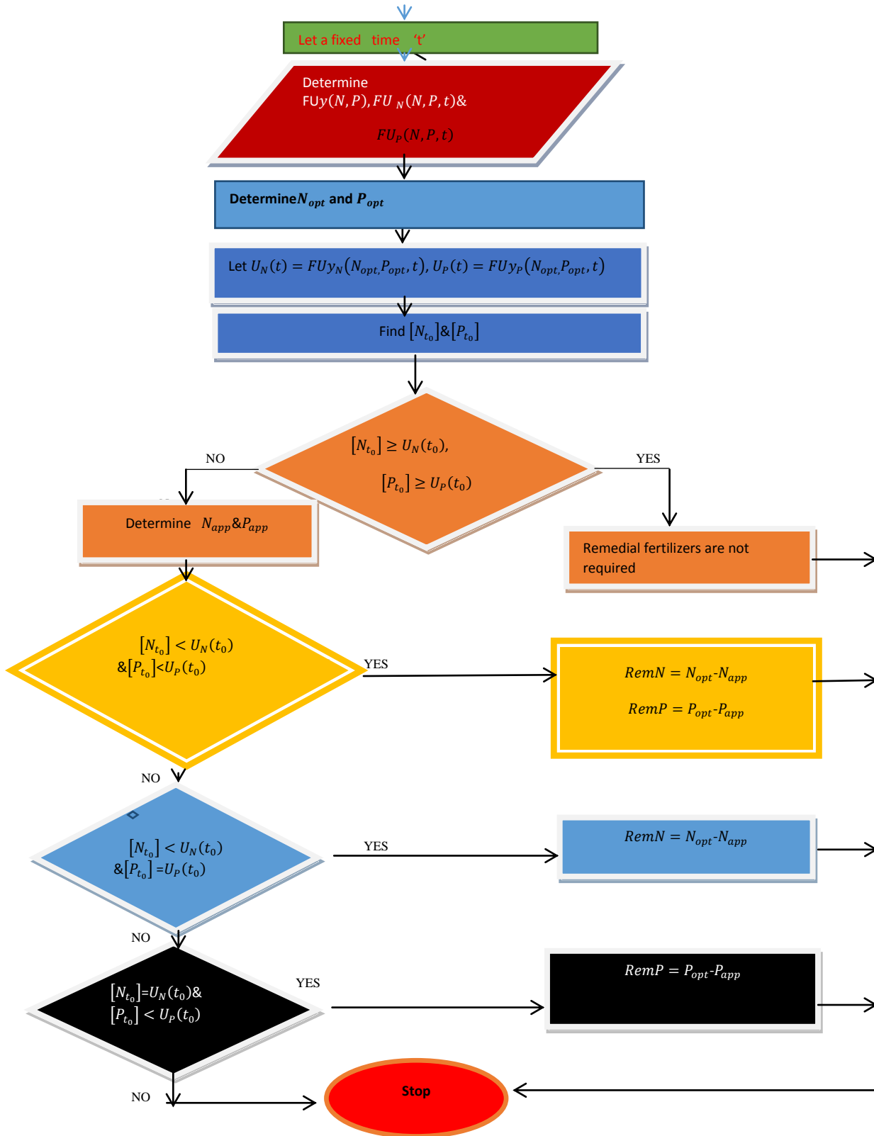
Fig.1. Algorithm of computational steps ( RemN : Remedial fertilizer of N , RemP : Remedial fertilizer of P )
