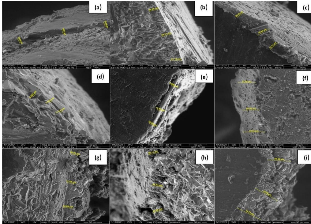
Figure 1. Scanning electron micrograph of (a) PSCU 5%, (b) PSCU 10%, (c) PSCU 15%, (d) POCU 2%, (e) POCU 4%, (f) POCU 6%, (g) HACU 5%, (h) HACU 10%, (i) HACU 15% at x1000 magnification.
