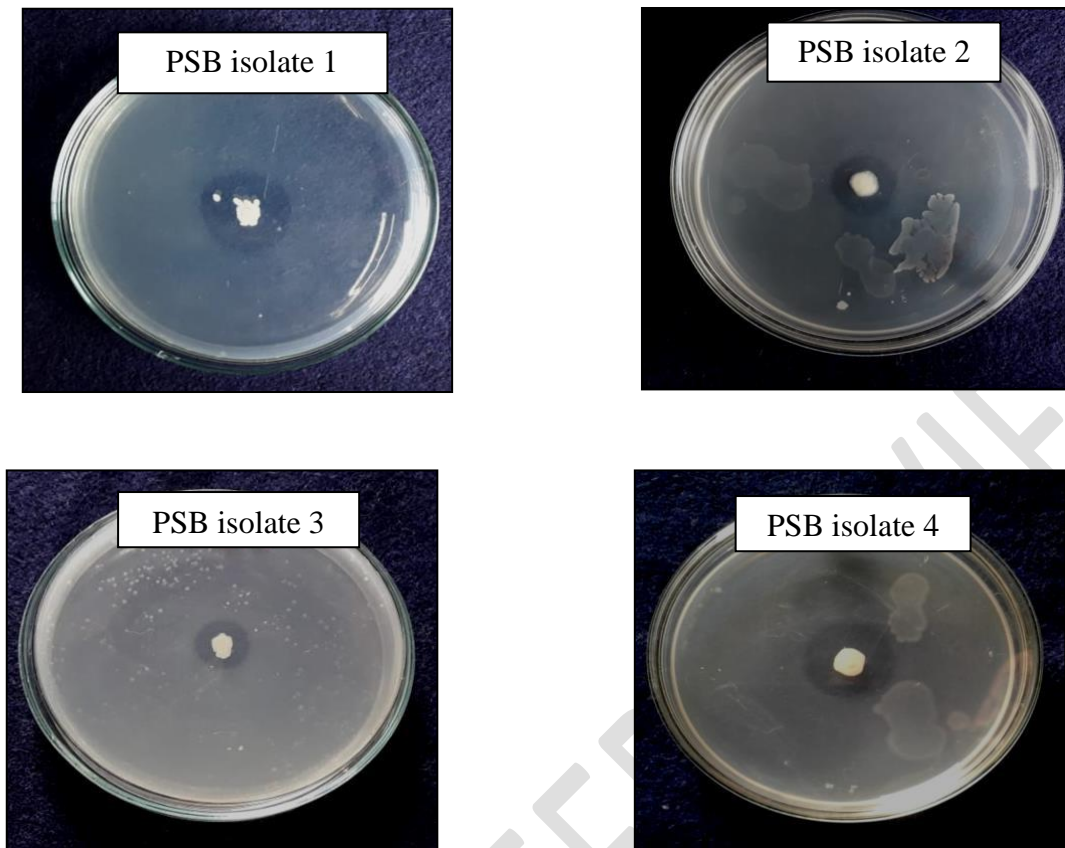
Fig 1. Formation of zone of solubilization on Pikovaskaya's agar plate by diff. effective PSB isolates.
