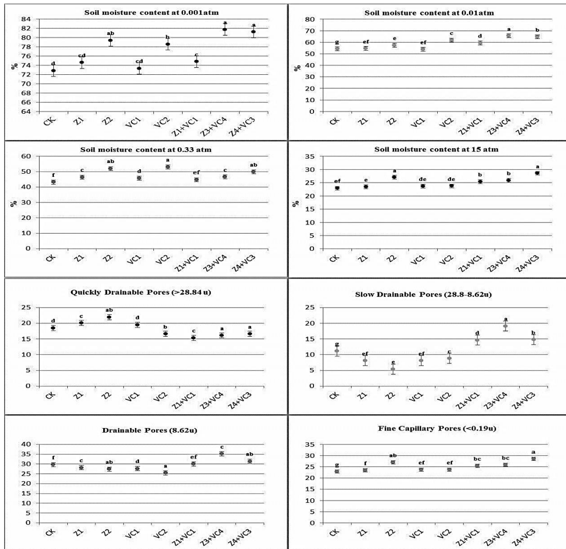
Fig.2. Effect of different rates of zeolite, vermicompost and their combinations on soil moisture content and pores size distribution after both seasons. Different letters on the top of the bars indicate significant differences at P < 0.05 .
