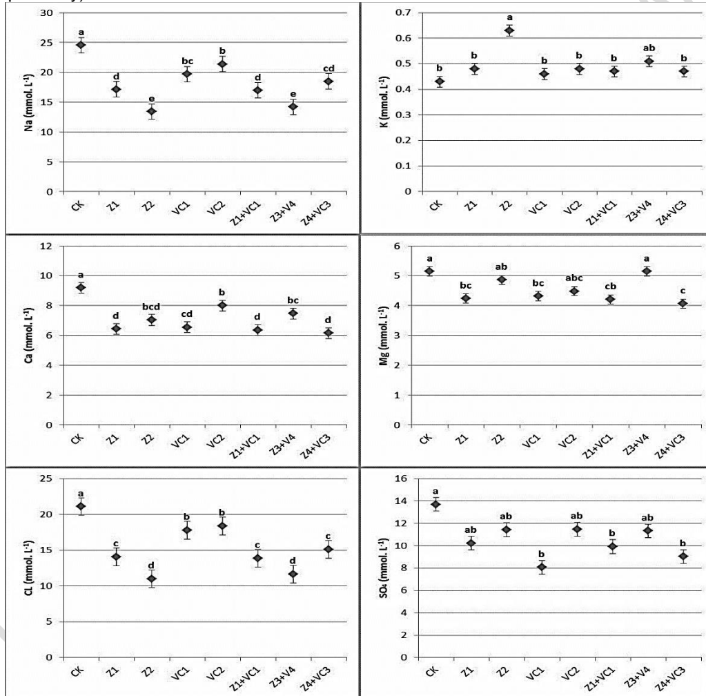
Fig.1. Effect of different rates of zeolite, vermicompost and their combinations on soluble ions. CK: Untreated soil (control), Z 1 : Zeolite applied at a rate of 1.20 Mg ha -1 , Z 2 : Zeolite applied at a rate of 2.40 Mg ha -1 , VC 1 : Vermicompost applied at a rate of 1.20 Mg ha -1 , VC 2 : Vermicompost applied at a rate of 2.40 Mg ha -1 , Z 1 +VC 1 : Zeolite: Vermicompost 1.20:1.20 Mg ha -1 , Z 3 +V 4 : Zeolite: Vermicompost 1.80: 0.60 Mg ha -1 and Z 4 +VC 3 : Zeolite: Vermicompost 0.60:1.80 Mg ha -1 , respectively. Different letters on the top of the bars indicate significant differences at P < 0.05.
