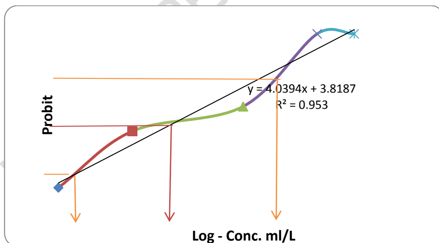
Fig. 2. Plot of probits versus log - concentration for calculation of LC 50 for Controller Super 2.5.
