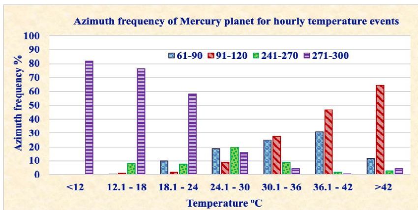
Fig 4. Azimuth frequency of Mercury planet for temperature events
