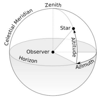
Fig. 2 Calculating Azimuth of the celestial body from the observer location
