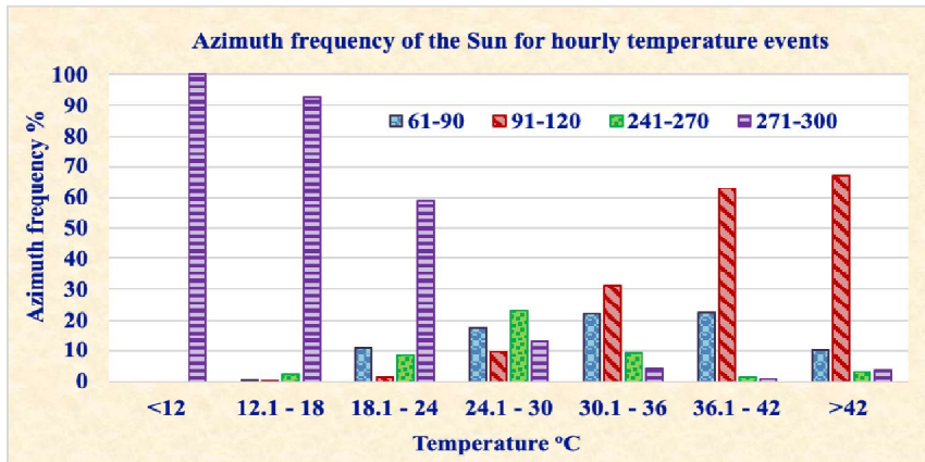
Fig 3. Azimuth frequency of the Sun for temperature events
