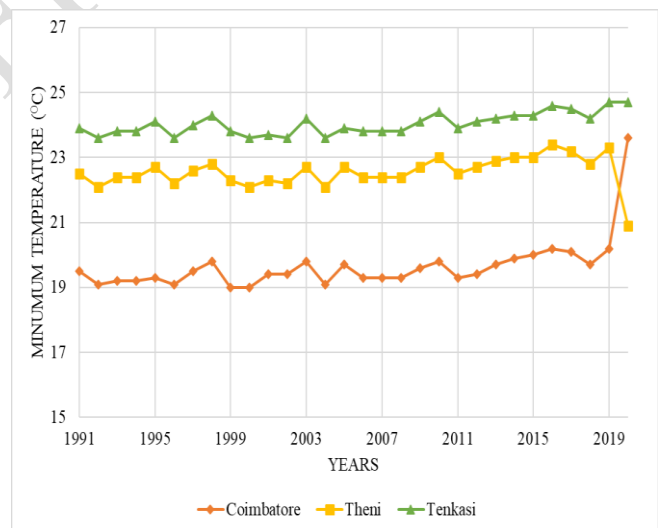
Fig. 7 Average minimum temperatures (°C) over study regions (1991 – 2020).
