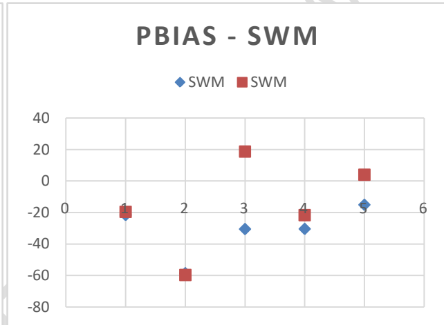
Fig. 3. PBIAS for WSM-3 and Kessler Scheme during SWM 2021
