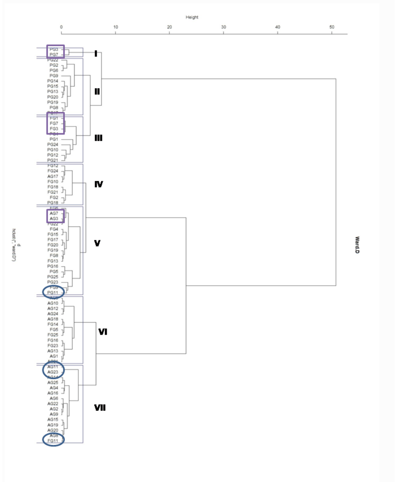
Fig.2.Results of hierarchical agglomerative cluster analysis based on photosynthetic nitrogen use efficiency in three treatments. The high PNUE and low PNUE genotypes in cluster are in frame.
