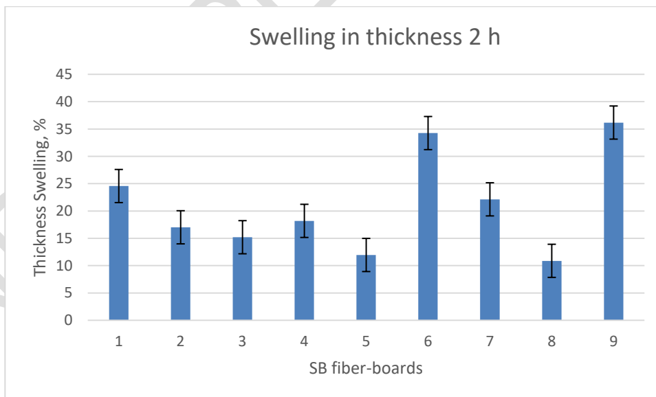
Figure.5 Thickness swelling values of fiber-boards immersed for 2 h
