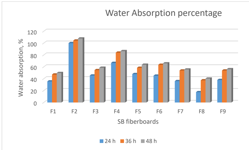
Figure.4 Percentage of water absorption by the samples immersed for 24 h, 36 h and 48 h.
