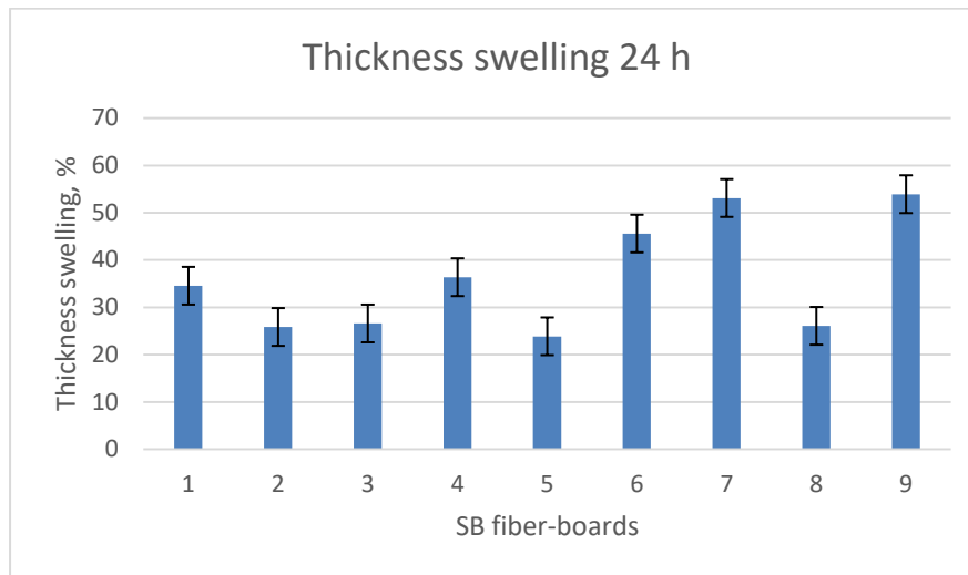
Figure.6 Thickness swelling values of fiber-boards immersed for 24 h
