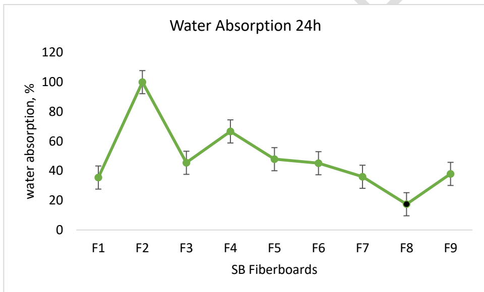
Figure.3 Percentage of water absorption by the fiber-boards immersed for 24 h
