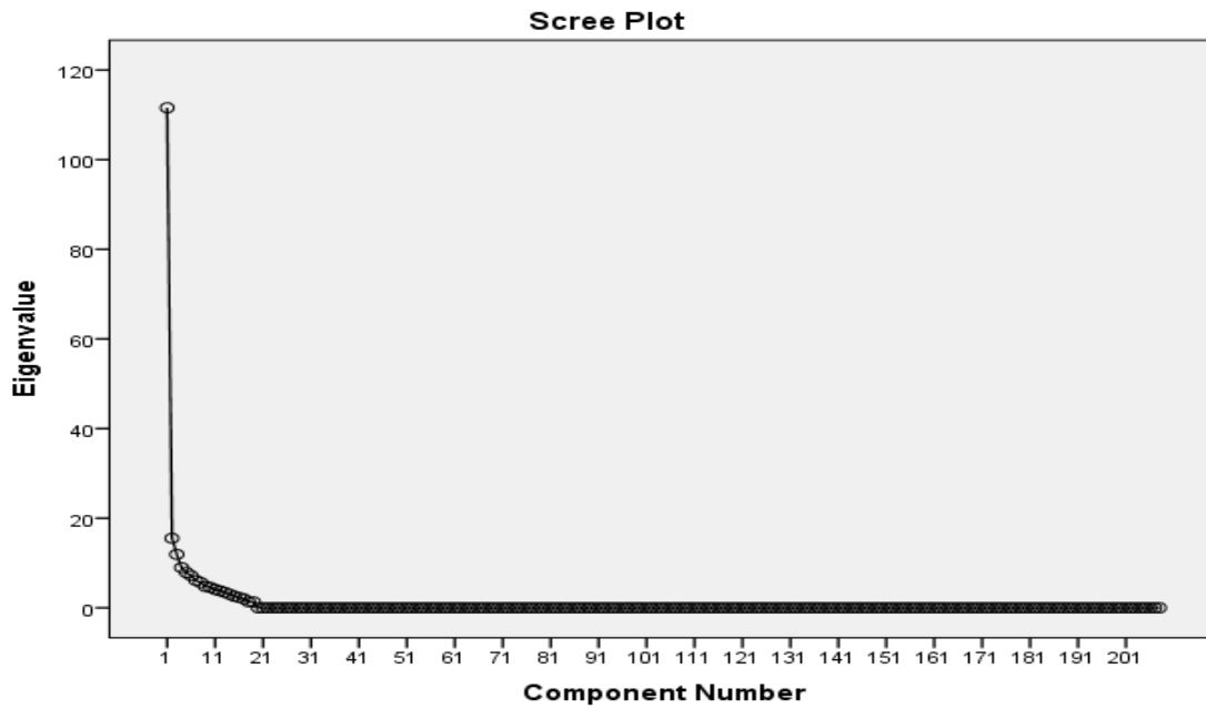
Fig 2. Scree plot obtained from PCA in SPSS
