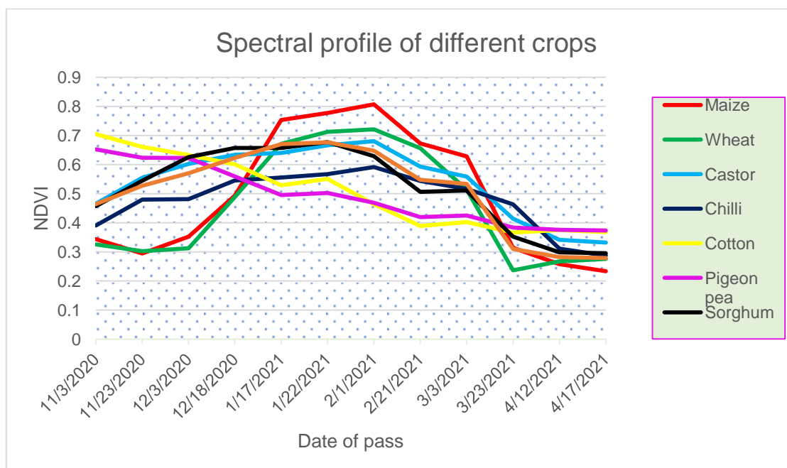
Figure 4 Spectral profile of different crops
