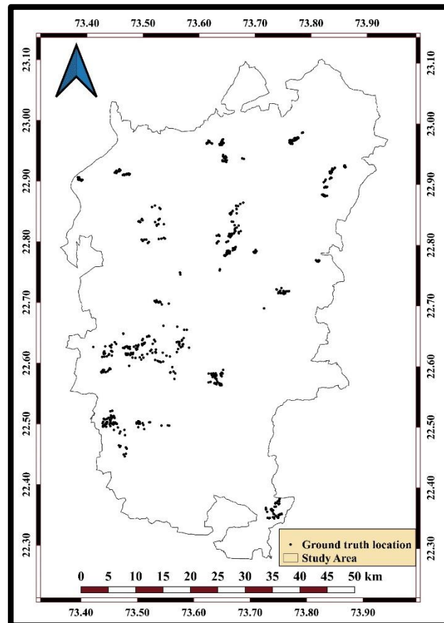
Figure 2 Spatial distribution map of ground truth locations
