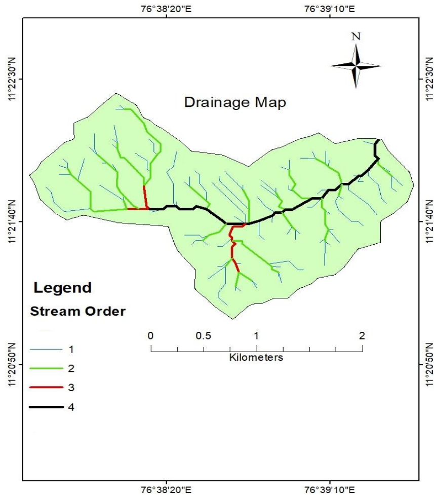
Figure 03: Stream order map
