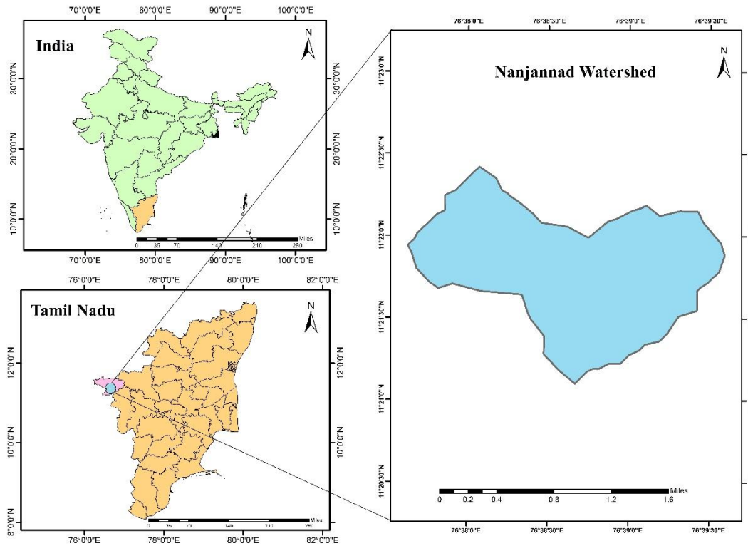
Figure 01: Nanjannad Watershed map
