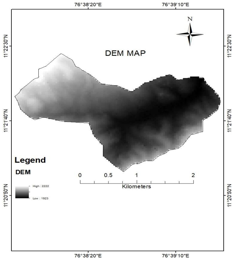
Figure 02: Digital elevation model (DEM) of Nanjannad Watershed
