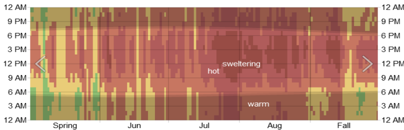
Image 1b: Wuhan Climate (Summer 2019) Hourly Temperature in the summer of 2019
