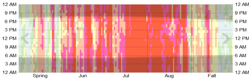
Image 1c: Wuhan Climate (Summer 2019) Humidity Levels in the summer of 2019
