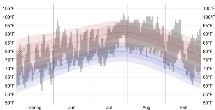
Image 1 a: Wuhan Climate (Summer 2019) Daily Temperature
