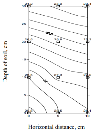
Fig. 8a : Moisture distribution under plastic mulch & dried leaves mulch next day after irrigation at 0.8 Epan
