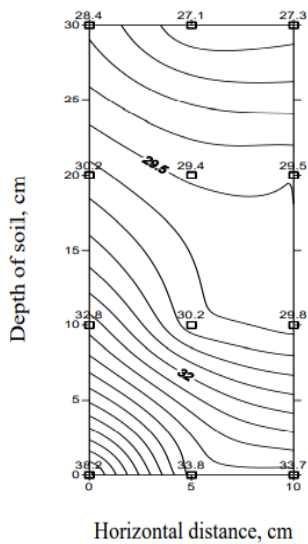
Fig. 2a: Moisture distribution under plastic mulch on the day of irrigation at 1.0 Epan
