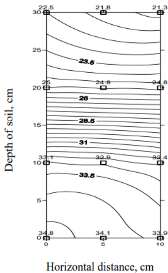
Fig. 4a : Moisture distribution under plastic mulch next day after irrigation at 1.0 Epan
