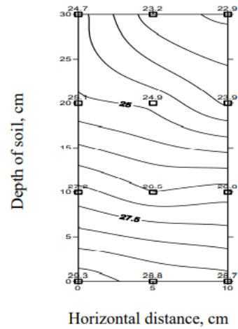
Fig. 1b: Moisture distribution under paddy straw on the day of irrigation at 1.0 Epan
