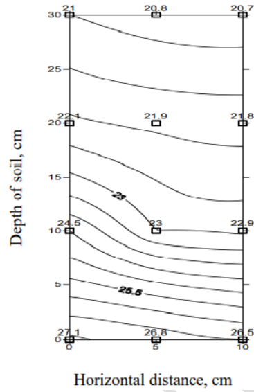
Fig. 6b : Moisture distribution under plastic mulch day & dried leaves mulch day of irrigation at 0.8 Epan
