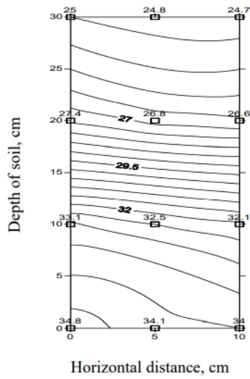
Fig. 6a : Moisture distribution under plastic mulch day & dried leaves mulch day of irrigation at 0.8 Epan
