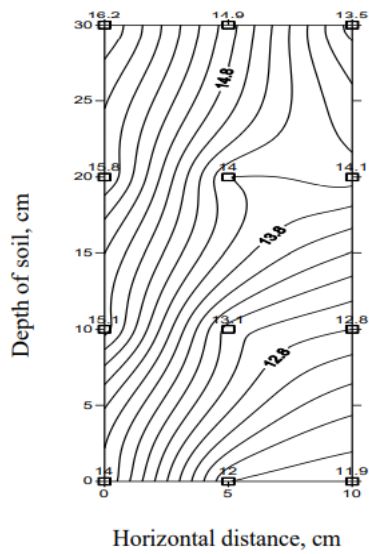
Fig. 11a: Moisture distribution under no mulch & paddy straw mulch next day after irrigation at 0.6 Epan
